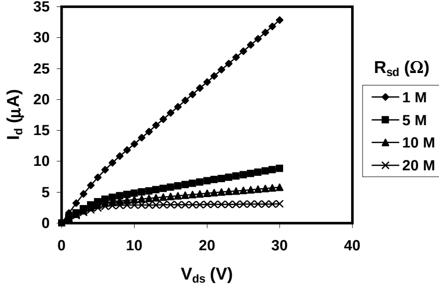
Figure 5.13: SPICE-generated I_d versus V_{ds} curves at a fixed V_{gs} with channel semiconductor resistance varying for a NiO:Li p-TTFT. In this simulation, R_{gs} and R_{gd} = 1\text{ G}\Omega , C_{gs} and C_{gd} = 1\text{ pF} , mobility \mu = 1\text{ cm}^2/\text{V}\cdot\text{s} , V_{gs} = 10\text{ V} , C_{ox} = 0.44\text{ F/cm} (for ATO gate insulator), and V_t = 2\text{ V} .
