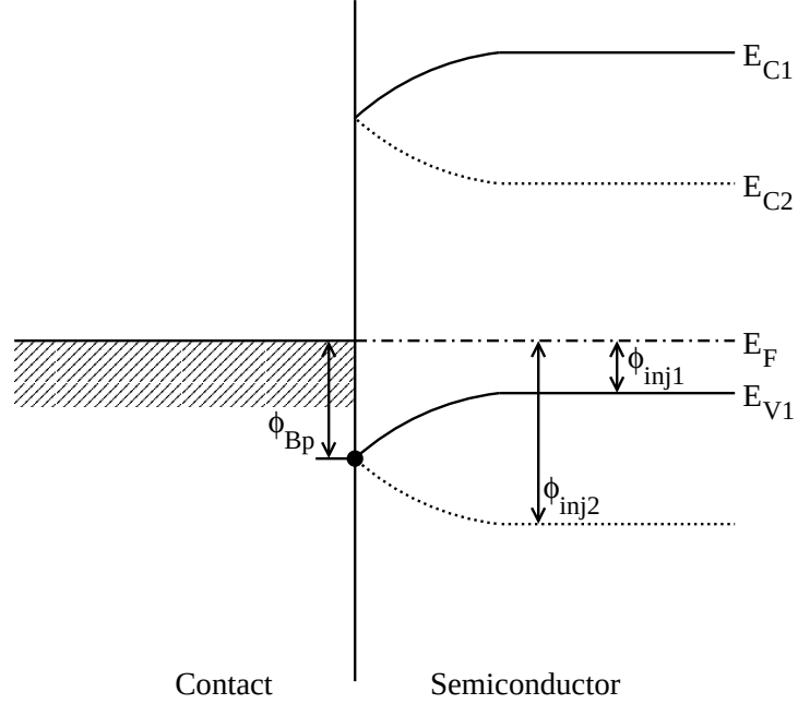
Figure 5.5: Equilibrium energy band diagram for a metal-semiconductor contact illustrating the change in hole injection barrier with semiconductor carrier concentration.
