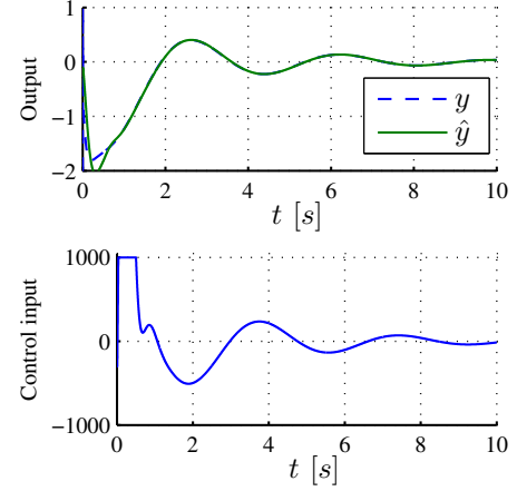
Fig. 3. Closed-loop performance with r = 2 and an optimized basis. Top: High-fidelity y and estimated \hat{y} . Bottom: eMPC control input, constrained such that |u| < 1000 . The input constraint is seen to be active during the first half second.
