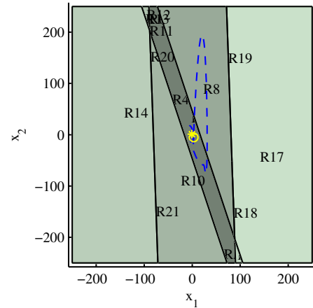
Fig. 4. Example of state-space partition for a reduced-order model with r = 2 , with state trajectory starting in o and ending in * . The different color shades indicate the 21 regions R_i in the state space. The controller feedback matrices (K_i, k_i) are constant within each region.
