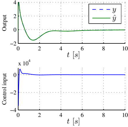
Fig. 1. Output-feedback LQ regulator for the high-fidelity model based on a reduced-order model with optimized basis for r = 3 . Top: Estimated output from the reduced-order model \hat{y} vs. output from the high-fidelity model y . Bottom: Control input.
