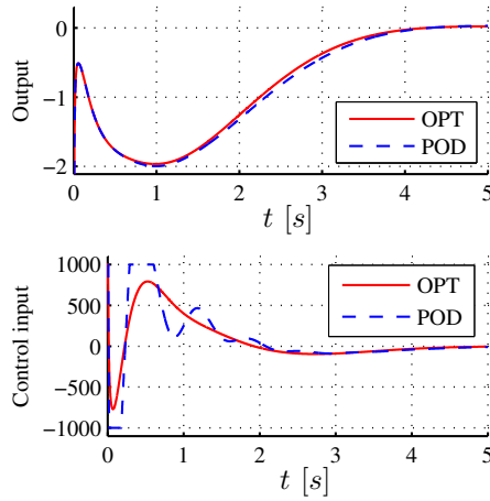
Fig. 5. Performance comparison for r = 5 with eMPC horizon N = 10 . Top: Output of the full model using reduced-order control based on optimized- and POD basis. Bottom: Control input for the two different cases.
