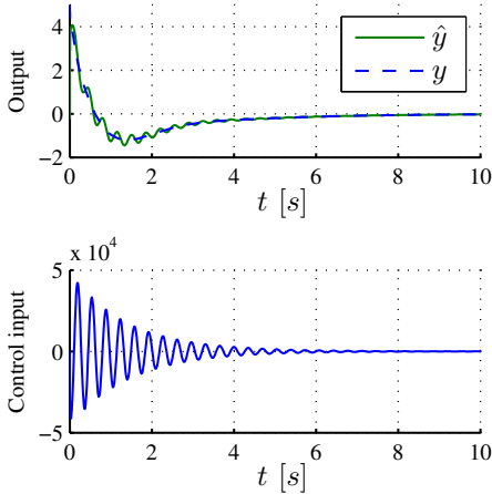
Fig. 2. Output-feedback LQ regulator for the high-fidelity model based on a reduced-order model with POD basis for r = 3 . Top: Estimated output from the reduced-order model \hat{y} vs. output from the high-fidelity model y . Bottom: Control input.
