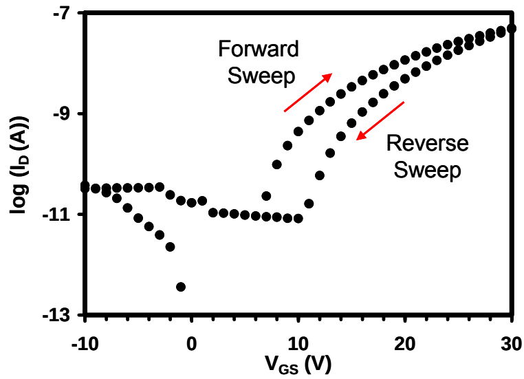
Figure 5.6: \log(I_D) - V_{GS} transfer curve with V_{DS} = 1 V showing clockwise hysteresis for a ZnO channel ( \sim 50 nm) TFT fabricated on thermal silicon oxide annealed at 200 °C is taken at t = 0 s. For the forward sweep, V_{ON} = 7 V, the reverse sweep gives V_{ON} = 11 V. The sweep rate is \sim 1 V/s.
