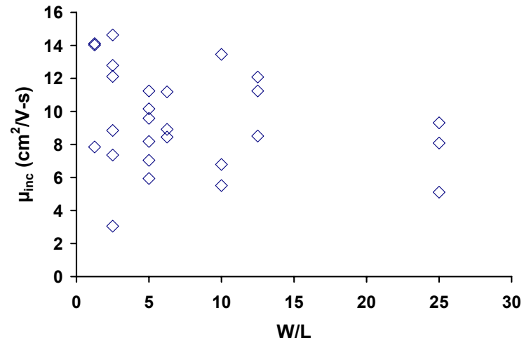
Figure 4.9: Maximum incremental mobility as a function of W/L for IGO ( \sim 50 nm) TFTs fabricated on \text{SiO}_2 and annealed at 600^\circ\text{C} .
