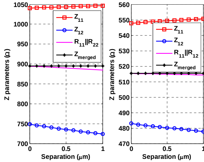
Figure 4.5. Comparison of Z-parameters from EPIC for merged single contacts with adjacent two contacts having contact dimensions (a) 1\mu\text{m} \times 1\mu\text{m} and 1\mu\text{m} \times 1\mu\text{m} , and (b) 5\mu\text{m} \times 5\mu\text{m} and 5\mu\text{m} \times 5\mu\text{m} .
