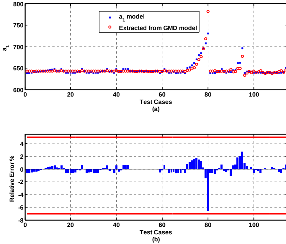
Figure 3.8. a_I as a function of geometry. (a) Comparison of the a_I model with extracted values from the GMD model. (b) Relative errors for the a_I model compared to the extracted values from the GMD model.
