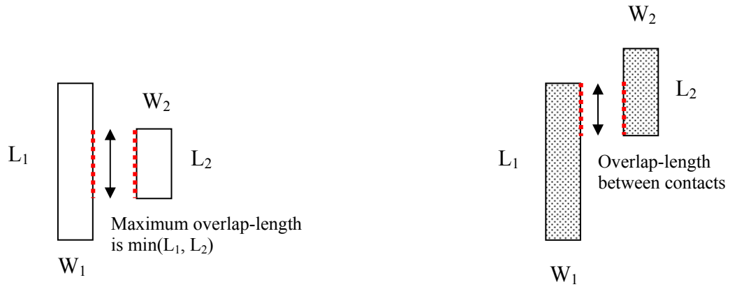
Figure 3.15. Overlap-length definitions.
