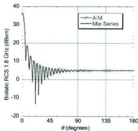
Figure 5. Scattering from a very large sphere.
