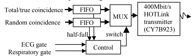
Figure 3: Sending coincidence data with HOTLink transmitter
