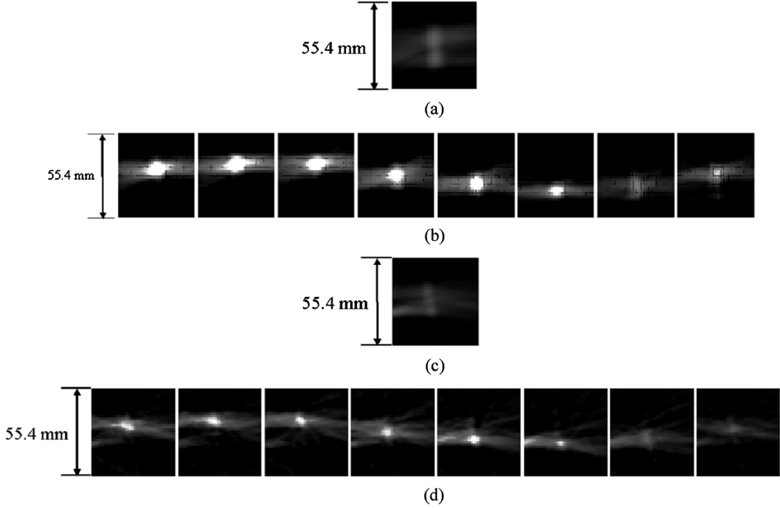
Fig. 6. Images of 5-mm and 3-mm lesion phantoms with and without respiration gating (same slice). (a) Nongated image of the 5-mm lesion phantom. (b) Respiration gated images of the 5-mm lesion phantom images. (c) Nongated image of the 3-mm lesion phantom. (d) Respiration gated images of the 3-mm lesion phantom images.
