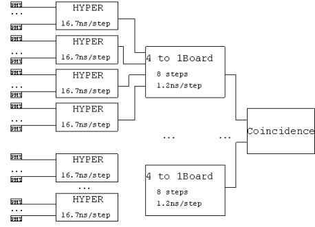
Fig. 5. Two programmable time alignment mechanism: coarse steps (16.7 ns/step) on the HYPER boards and fine steps (1.2 ns/step) on the 4-to-1 boards.
