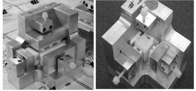
Fig. 7. (a) Gluing jig with sandwich compressed in three dimensions. (b) Final PSSDA inside the jig with the top compression piece removed.
