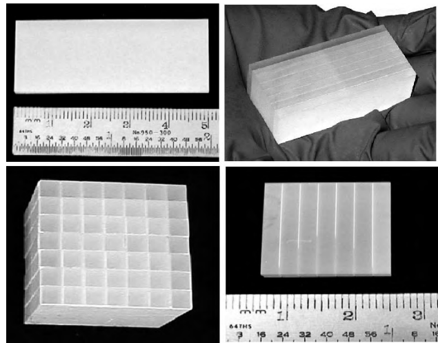
Fig. 4. Pictures showing the four stages of the SSS production process. Clockwise direction (from top left): slab, sandwich, slice, and 7 \times 7 PSSDA.
