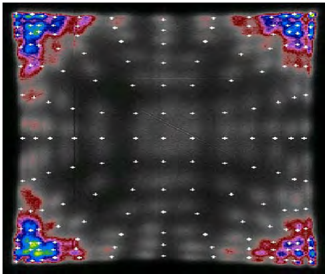
Fig. 7: Comparison of the expected crystal positions from the simulation software (white points) with the experimental crystal decoding map (background image).
