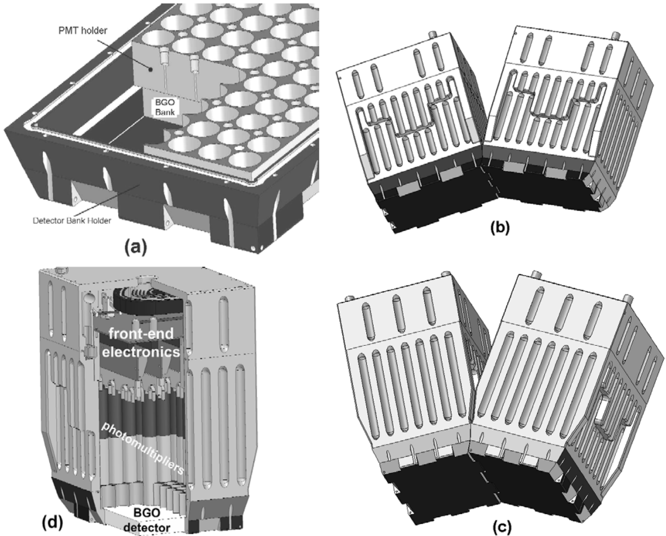
Fig. 4. HOTPET's detector module and its configurations. (a) Detector-bank-holder . (b) Short sides of the rectangular holder are mated together forming a 30^\circ angle and a large-diameter polygon for whole-body imaging. (c) Long sides of the rectangular holder are mated together forming a 30^\circ angle and a small-diameter polygon for brain/breast mode. (d) Detector module internal components.
