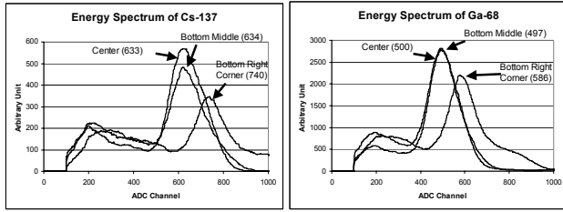
Figure 8. Lapped Type . Energy spectra for 3 individual crystals (center, bottom middle, bottom right corner) using (Left) ^{137}\text{Cs} source, (right) ^{68}\text{Ga} source.
