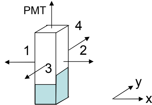
Fig.5: Definitions of optical windows for each crystal. Light can go through the four side optical windows to its neighbor crystals or pass to the direct PMTs through the top window.
