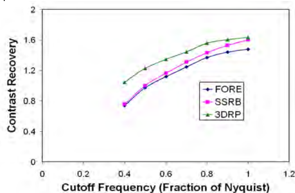
Fig. 5. Contrast recovery for the 6 mm lesion using the Hamming apodization function as a function of the cutoff frequency. The lines simply connect the points.
