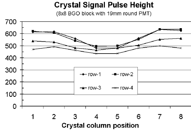
Fig. 8. Raw pulse-height distribution for 8 \times 8 array with 19 mm PMT.
