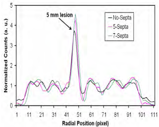
Fig. 8. Horizontal profiles through the middle of the images of the 5 mm hot lesion in cold background for no-septa and partial-septa configurations. Activity concentration of the 5 mm lesion was the same as data in Fig. 7.
