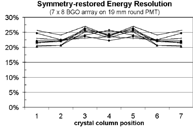
Fig. 15. Symmetry-restored energy resolution distribution for 7 \times 8 array.
