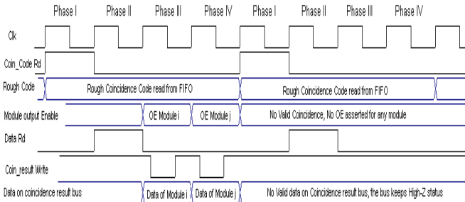
Fig. 5 Timing diagram of the second level coincidence processing logic (module number i < j , i, j \in 1, \dots, 12 )
