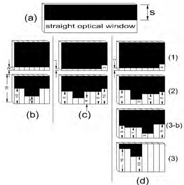
Fig. 5. Examples of slab and slice paint-masks used for HOTPET. (a) Masks for slabs that make up a sandwich; straight masks with constant height “s” covering the length of the slab. (b) Masks for slices of symmetric PSSDA (middle blocks Fig. 1). (c) Masks for slices of extended arrays placed at the edge of the detector module in Fig. 1. (d) Masks for the corner arrays of the same module.
