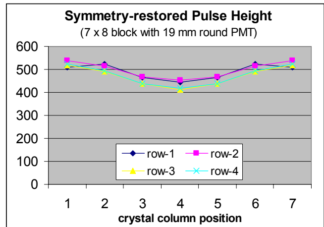
Fig. 12. Pulse-height distribution for the 7x8 array with 19mm PMT
