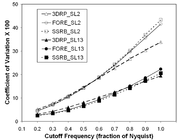
Fig. 2. CV for an edge slice (slice no. 2) and a central slice (slice no. 13) as a function of the cutoff frequency. The lines simply connect the points.
