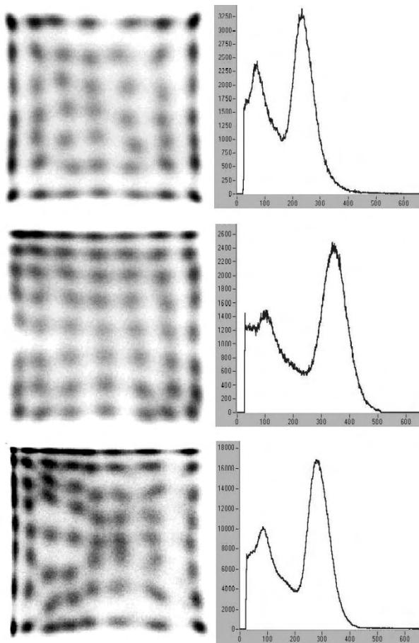
Fig. 9. Two-dimensional decoding map (left) and composite energy spectra (right) of all needles from the three types of PSSDA used in HOTPET (Fig. 1). (Top) 7 \times 7 symmetrical array, (middle) 7 \times 8 extended nonsymmetrical array, (bottom) 8 \times 8 optically nonsymmetrical array used for the module's corners. (Electronic gain and PMT high-voltage settings not equal for all configurations).
