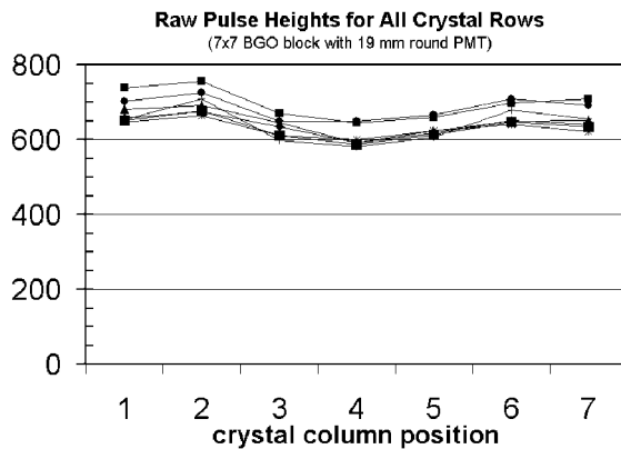
Fig. 3. Raw crystal pulse-heights for all seven rows of crystals.
