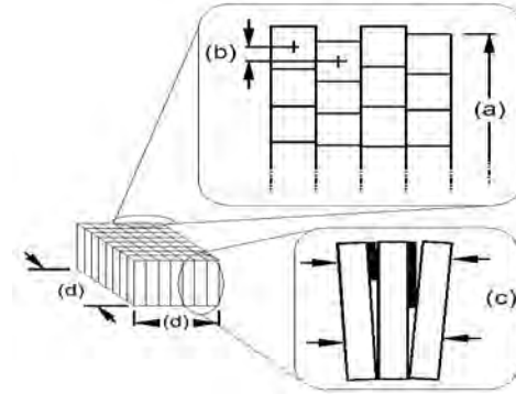
Fig. 8. Fours sources of mechanical tolerances from the SSS manufacturing process: (a) glue, paint and slab thickness (needle positioning error; measures repeatability.); (b) systematic differences between sandwich types; (c) needle slant (gluing jig limitations, paint placement); (d) axial vs. trans-axial dimension differences (size of surface glued).
