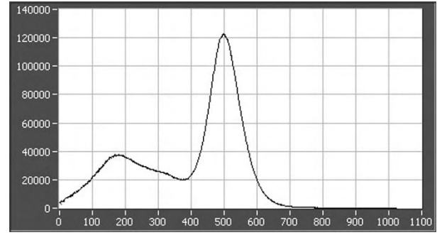
Fig. 12. Array-average spectrum for the 2.3 mm \times 2.3 mm \times 10 mm BGO.
