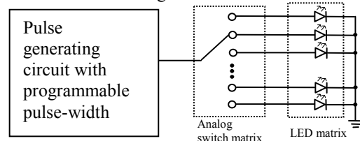
Fig. 5: Only one computer-programmable pulse generator is needed to drive the LED network.
