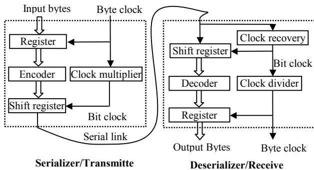
Figure 1: HOTLink architecture
