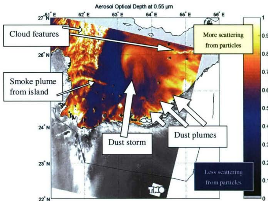
Figure 3.7 The Aerosol Optical Depth for 0.55 μm over water on September 7, 2004 during the United Arabic Emirates Unified Aerosol Experiment. Part of the Persian Gulf is visible. Many atmospheric features are visible, like clouds, smoke, dust plumes and a dust storm – all aerosols. The AOD product has been obtained by using a dedicated retrieval algorithm that uses a two-type modelled aerosol mixture to be compared with the signal at the satellite sensor. The AOD can be retrieved for four wavelengths and indicated the amount of scattering (in this case, as only scattering aerosol types have been modelled).
