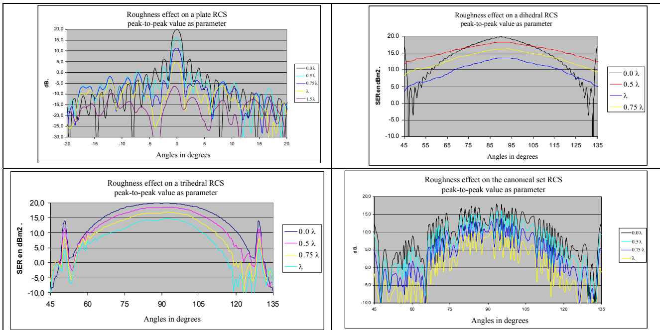
Figure 6: Roughness effect on RCS of canonical targets
