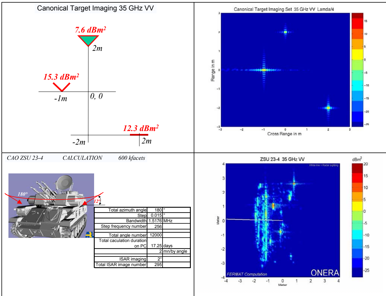
Figure 3: Examples of ISAR images from the canonical target set and the ZSU 23-4
