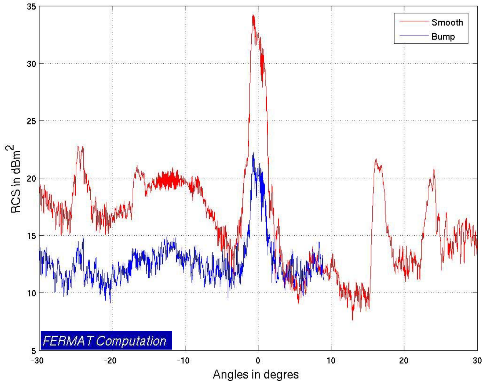
RCS ZSU 23-4 60k 35 GHz VV (frequency mean)
