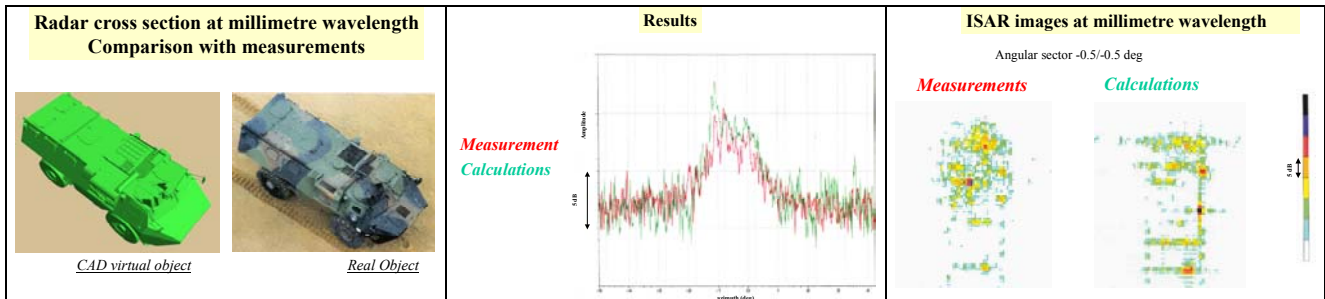
Figure 4: Previous results in using roughness texture on a recovery vehicle
