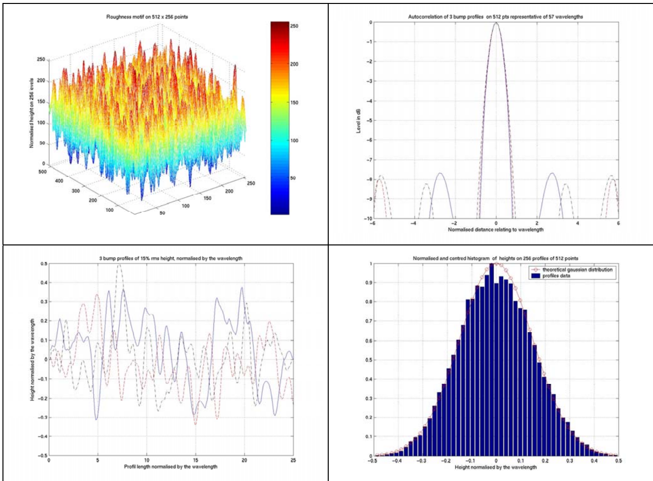
Figure 5: Statistical profile parameters
