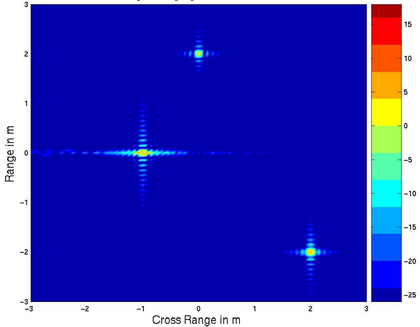
Canonical Target Imaging Set 35 GHz VV \lambda/4
