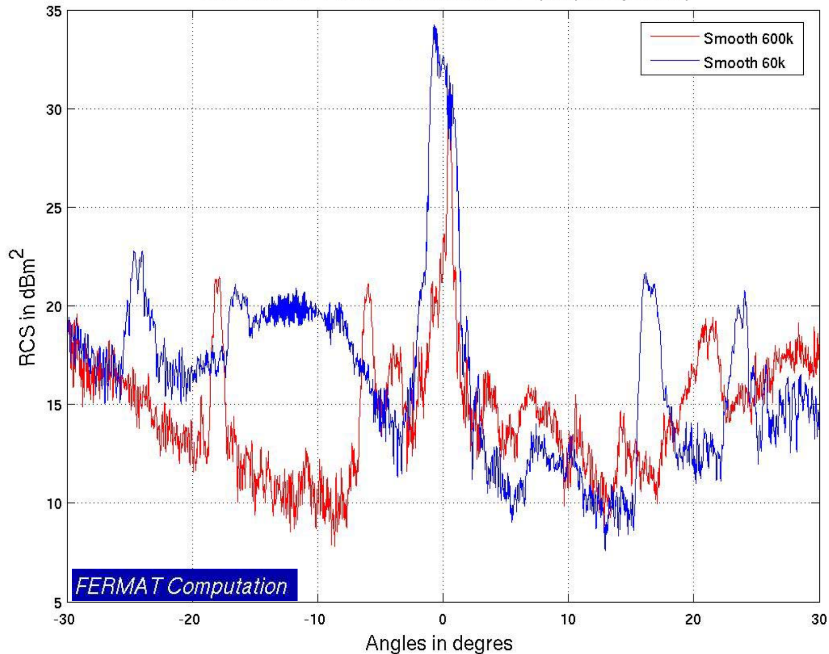
RCS ZSU 23-4 600k / 60k 35 GHz VV (frequency mean)
