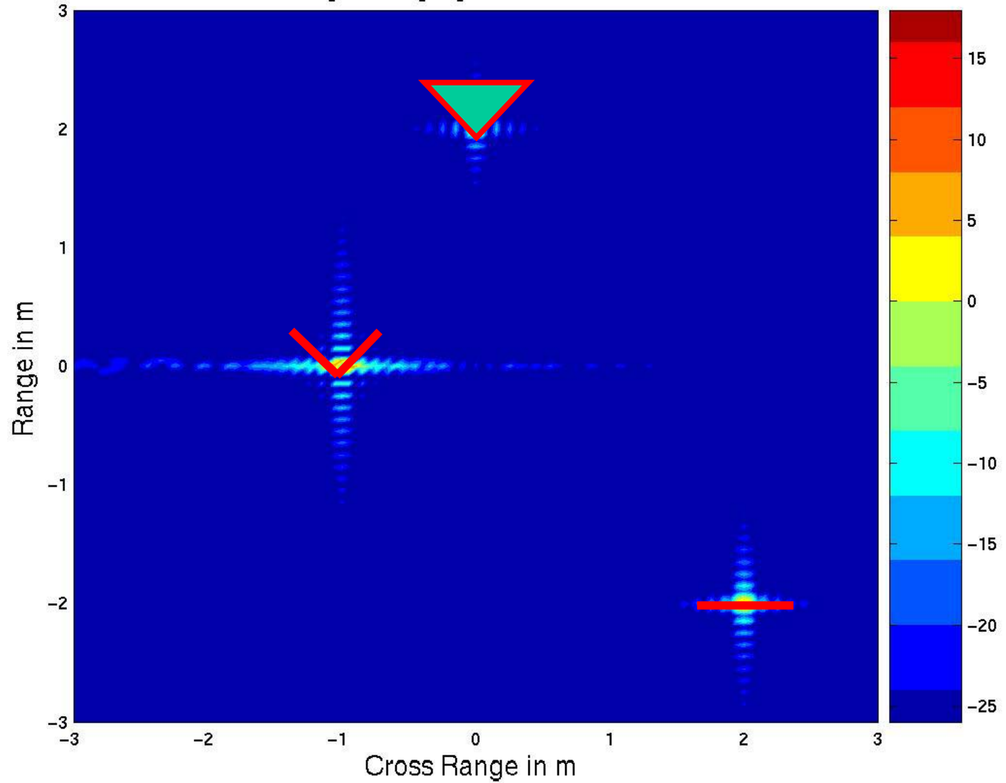
Canonical Target Imaging Set 35 GHz VV Lamda/4
