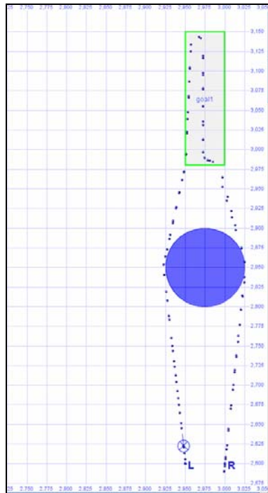
Figure 31. Agenda Mission where the vehicle has to avoid the circle, obstacle area, search the rectangle and return. The dotted-line track indicates successful completion from launch to recovery point.
