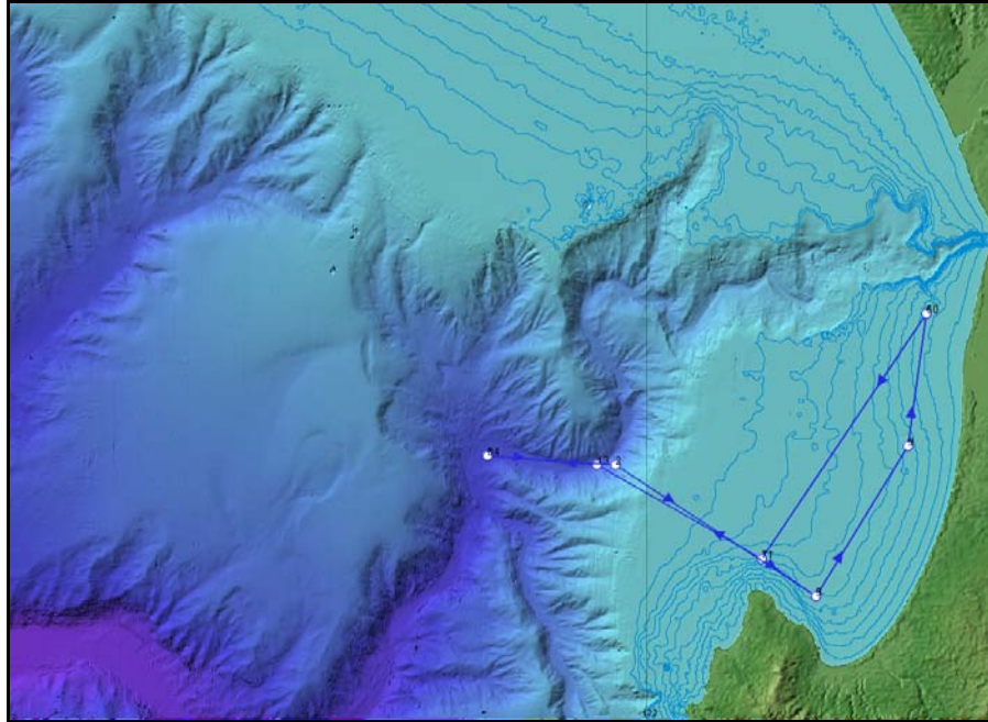
Figure 35. Intelligence Surveillance Reconnaissance mission in the Open Map view, showing proximity to the surveyed area and the use of the deep channel for covert launch and recovery.
