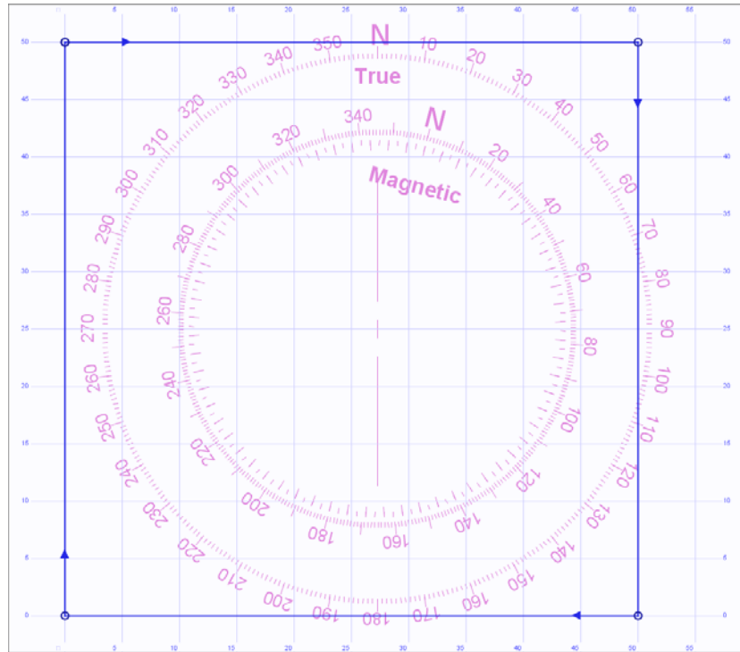
Figure 29. A screen shot of a scripted mission from the AUVW 2D mission planner with a compass rose
