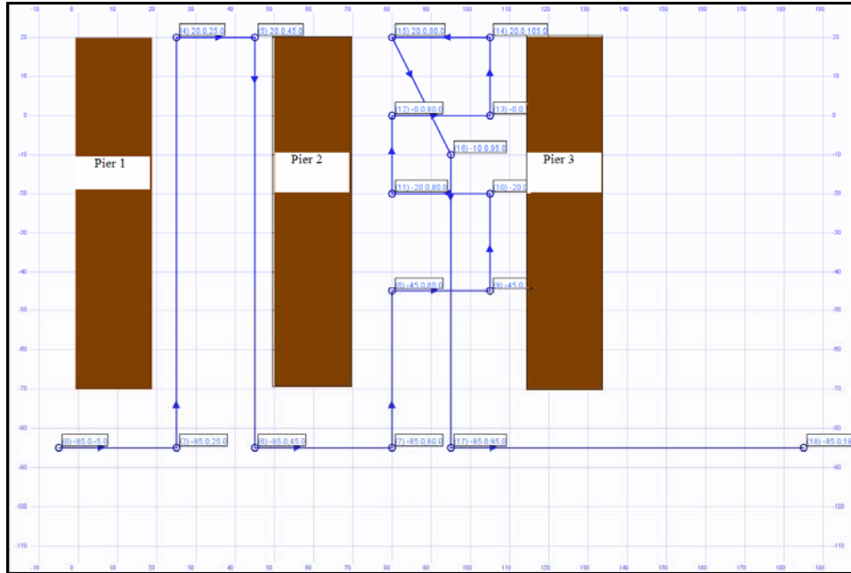
Figure 42. The Inspection and Identification mission with piers over the mission plan.
