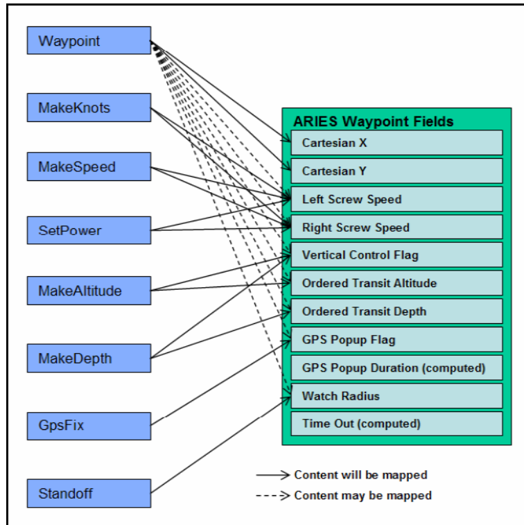
Figure 24. This illustrates AVCL to the ARIES waypoint command translate from (Davis 143)
