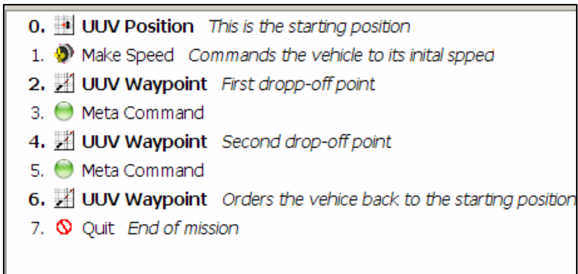
Figure 48. The AVCL commands for the payload mission
