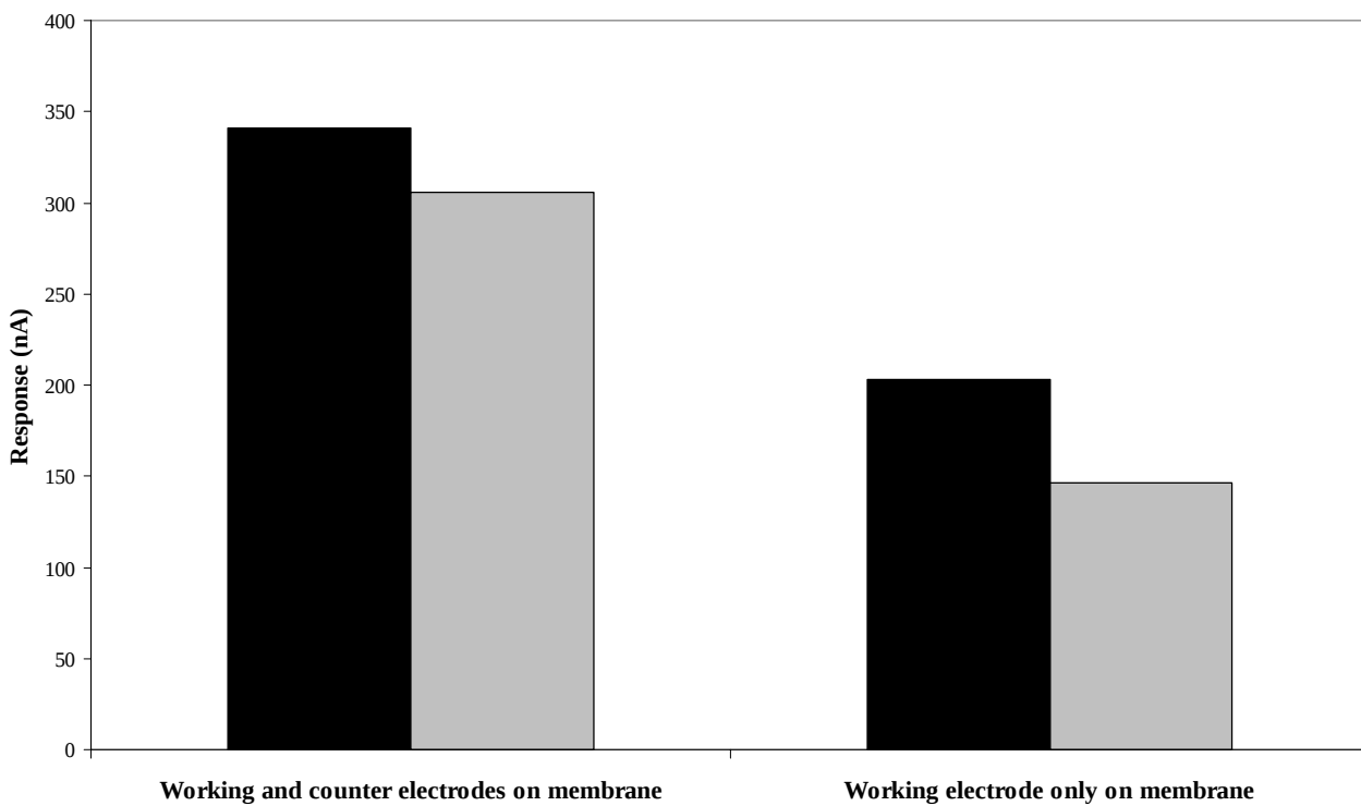
Figure 7: Comparison of sensor response for 1.69 mM acetylthiocholine, 0.013 U AChE, phosphate buffer (pH=7.4) solution with the working electrode only on the nanoporous membrane and the working and counter electrodes in tandem on the membrane. Black bars represent immobilized AChE, while grey bars represent AChE free in solution.
