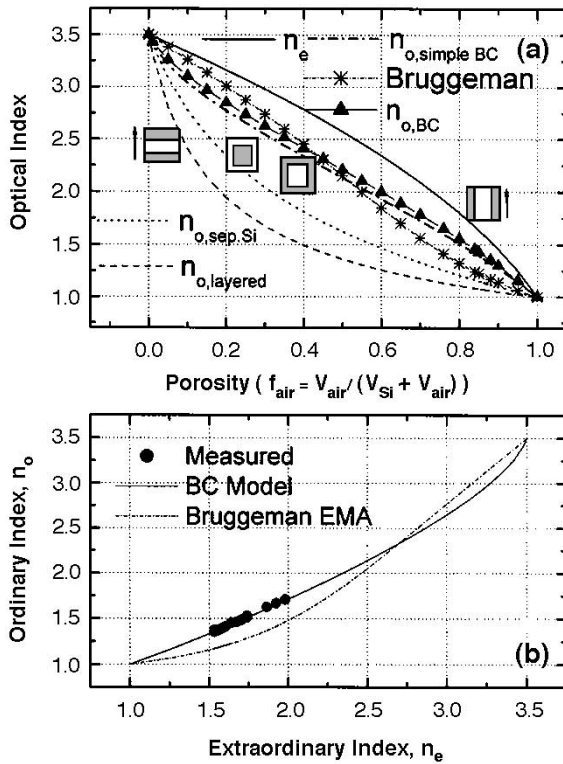
Fig. 3. Comparison of (a) index curves from various models as a function of porosity and (b) index pair coordinates of (n_e, n_o) in the index plane. Four different diagrams in (a) denote simplified microscopic geometric arrangements of pores. The arrow represents the direction of the electric field.
