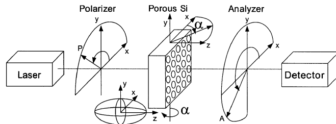
Fig. 1. Schematic diagram of experimental setup and the index ellipsoid of a Psi film.
