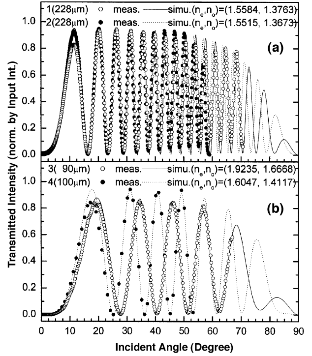
Fig. 2. Comparison of the polarization interference signals through a porous silicon film as a function of incident angle (a) for two films of same thickness of 228 \mu\text{m} with slightly different porosity of 0.875 and 0.873 and (b) for two films of similar thicknesses of 90 and 100 \mu\text{m} , but with quite different porosity of 0.86 and 0.76.
