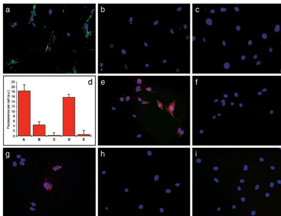
Fig. 2. Binding of peptide-conjugated qdots to endothelial cells and breast cancer cells in vitro is specific to peptide sequence. ( a ) Binding of green GFE-conjugated qdots to LE cells that express membrane dipeptidase. ( b and c ) Inhibition of GFE-qdot binding to LE cells by free GFE peptide (500 \mu M) ( b ) or with cilastatin, an inhibitor of the receptor, membrane dipeptidase (50 \mu M) ( c ). ( d ) Quantification of fluorescence intensity of an experiment similar to the one illustrated in a – c . (Columns A–C) GFE-qdot binding to LE cells; GFE concentration 250 \mu M; and cilastatin 50 \mu M. (Column D) The binding of GFE-qdots to the LE cells is not inhibited by a control peptide (LyP-1; 250 \mu M). (Column E) LyP-1-qdots do not bind to the LE cells. The fluorescence associated with 10 individual cells from each panel was measured by using digital image analysis. Background fluorescence from cells that received no qdots has been subtracted (2 a.u., arbitrary units). A representative experiment of five experiments was quantified. ( e and f ) F3 qdots bind to MDA-MB-435 breast carcinoma cells ( e ); free F3 peptide (500 \mu M) inhibits the binding ( f ). ( g ) Binding of LyP-1 qdots to MDA-MB-435 cells. ( h and i ) GFE qdots do not recognize the MDA-MB-435 cells ( h ) and LyP-1 qdots do not bind to the LE cells ( i ). Nuclei were visualized with 4',6-diamidino-2-phenylindole staining (blue). Cells were examined under an epifluorescence microscope with a 425/40-nm excitation and a 515-nm long-pass filter. (Original magnifications: a – c and i , \times 200 ; and e – h , \times 400 .)
