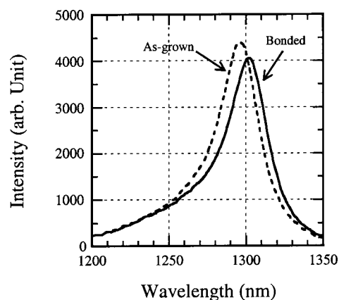
FIG. 4. PL spectra from the active region. Broken line: As grown on (311)B InP, solid line: Bonded onto GaAs substrate.
