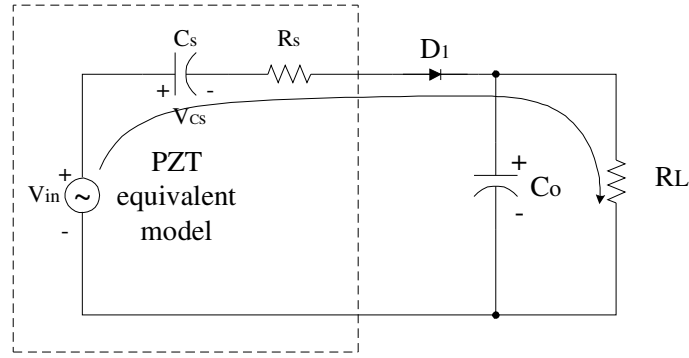
(a) Without R_c
