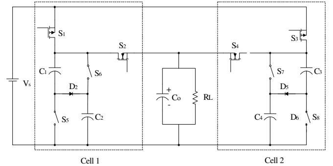
(a) Circuit
