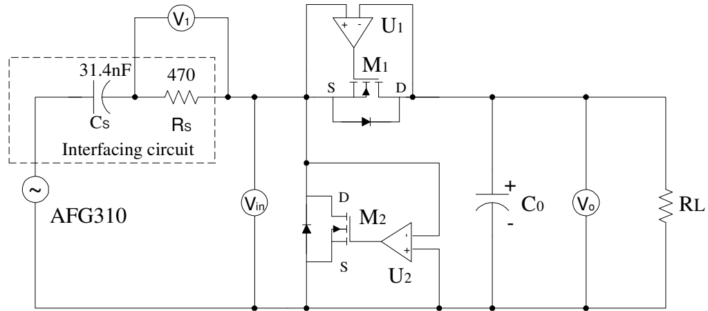
Fig. 6.5. AWGR connected to scheme III.
