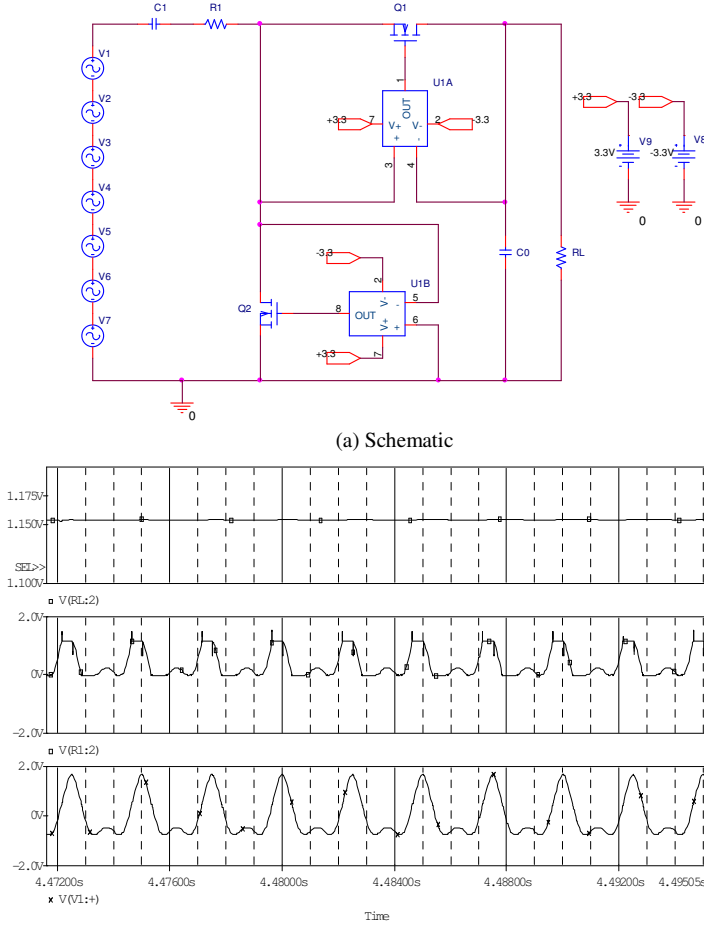
Fig. 8. PSpice simulation for scheme III.
