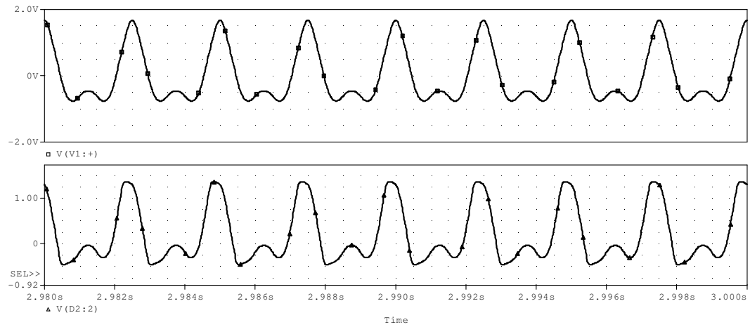
(b) Upper: PZT model terminal voltage waveform during no load Bottom: PZT model terminal voltage waveform for an 80\text{k}\Omega resistive load
