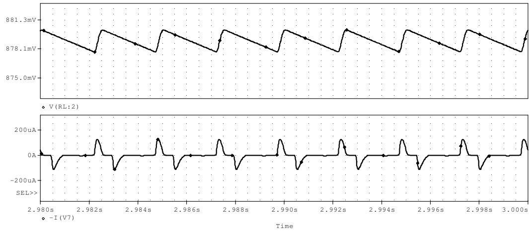
(a) Upper: output voltage waveform for an 80\text{k}\Omega resistive load Bottom: input current waveform for an 80\text{k}\Omega resistive load
