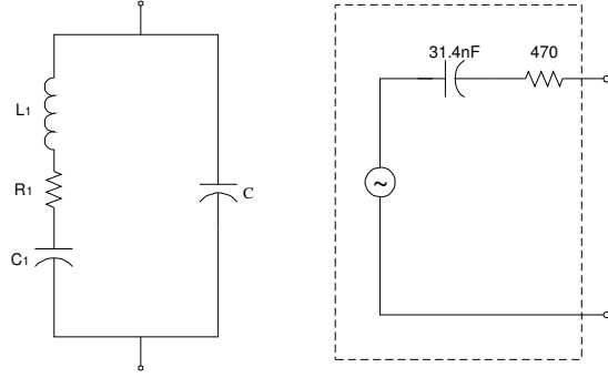
(a) Van Dyke's model (b) Simplified model Fig. 4. Equivalent model of the piezoelectric generator.
