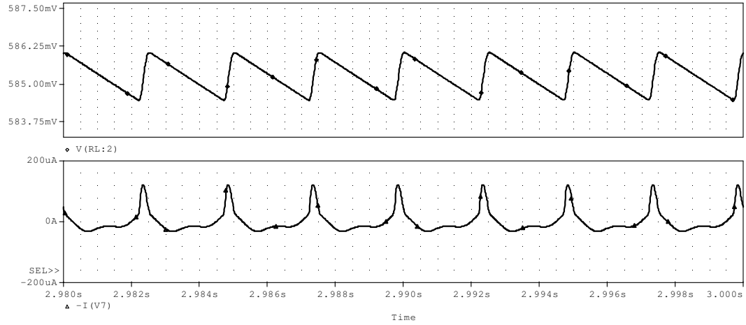
(a) Upper: output voltage waveform for an 80k\Omega resistive load Bottom: input current waveform for an 80k\Omega resistive load
