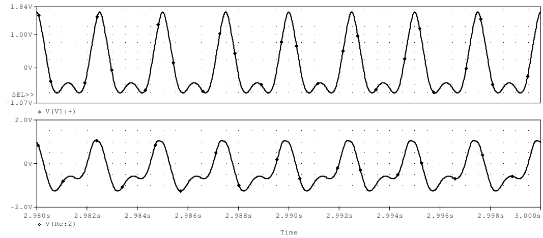
(b) Upper: PZT model terminal voltage waveform during no load Bottom: PZT model terminal voltage waveform for an 80k\Omega resistive load
