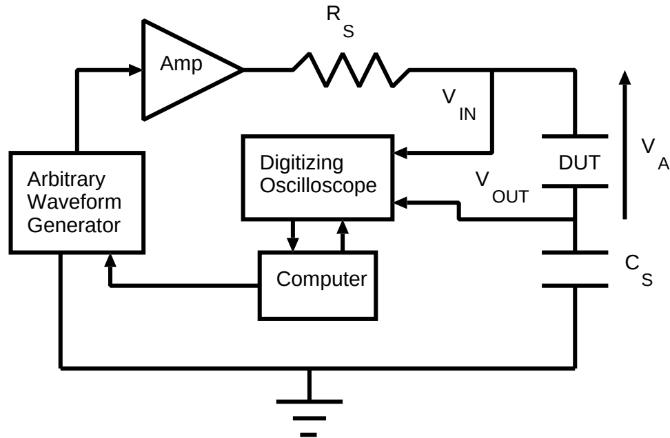
Figure 3.3: Sawyer-Tower circuit used for ferroelectric device characterization.
