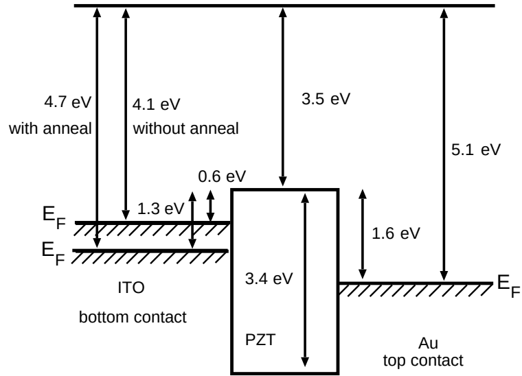
Figure 4.1: The barrier to electron injection from ITO can be improved by annealing.
