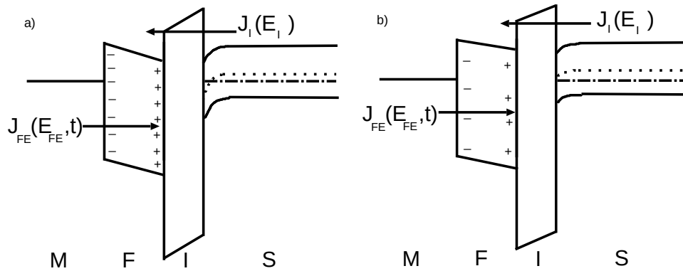
Figure 2.13: Gate leakage effects in MFIS devices. (a) Inverted semiconductor immediately after polarization, and (b) depolarization after time.
