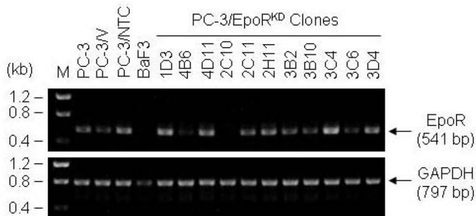
Figure 11. Semi-quantitative RT-PCR to determine EpoR expression levels in PC-3 cells stably transfected with EpoR shRNA constructs (PC-3/EpoR KD ). Cells transfected with none (PC-3), with vector only (PC-3/V) and with non-targeting control plasmid (PC-3/NTC) were included as positive controls. BaF3, not expressing human EpoR, was used as negative control. DNA size marker (M) is labeled to the left and the expected sizes of EpoR and GAPDH products are indicated to the right.
