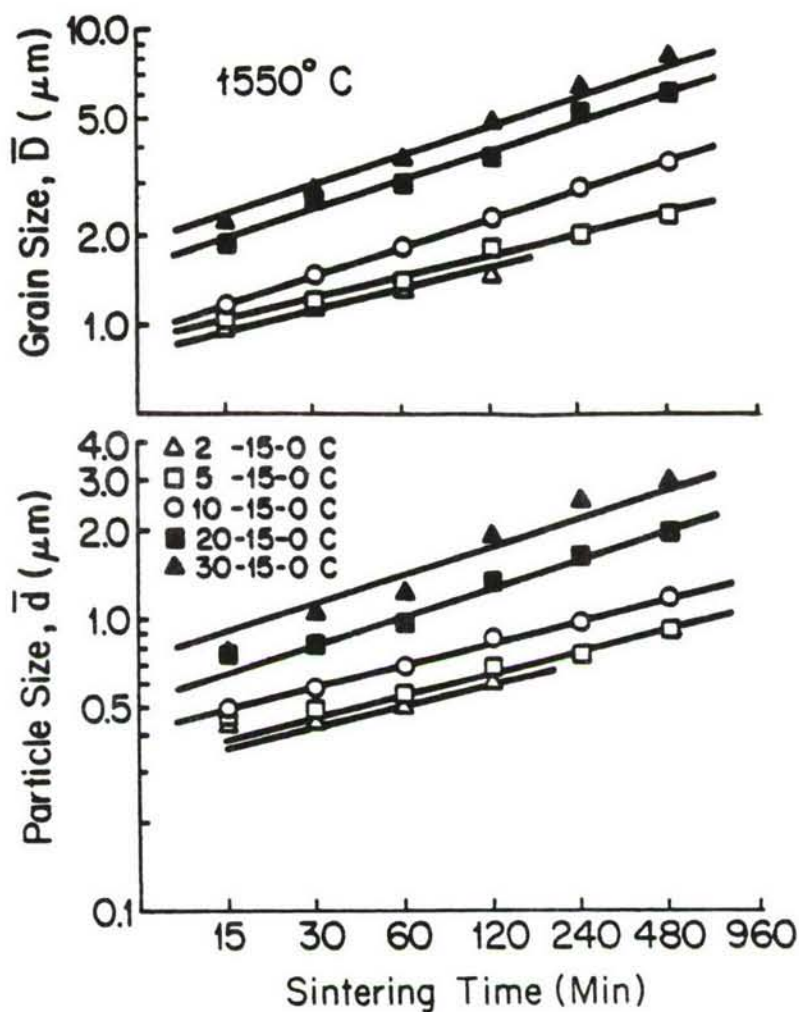
Fig. 2. Grain and Particle Growth Data for Composites Sintered at 1550°C., Starting Powder Used: "C" - Alpha Alumina Composition Designation: \text{Cr}_2\text{O}_3 Content - Vol % \text{ZrO}_2 - \text{HfO}_2 Content - Starting Powder.
