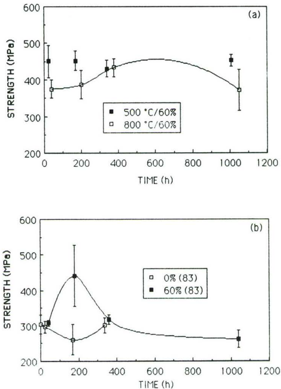
Figure 1. Strength behavior obtained for TS(83) PSZ at 500°C (a) was insensitive to time while data obtained at 800°C (a) and 1000°C (b) gave evidence of an applied stress dependence.
