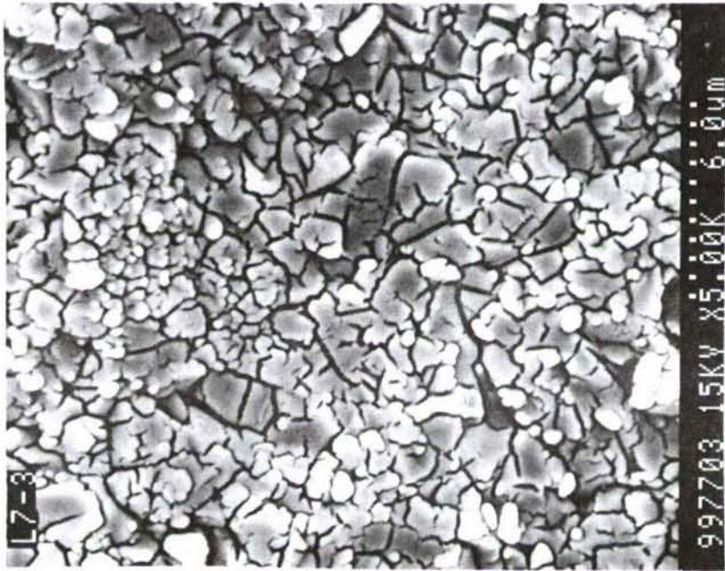
FIGURE 19 FRACTURE SURFACE COMPOSITE NO. 7
