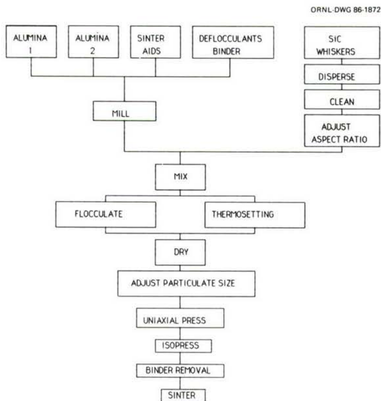
Fig. 1. Summary of fabrication route for pressureless-sintered alumina-SiC whisker composites.
