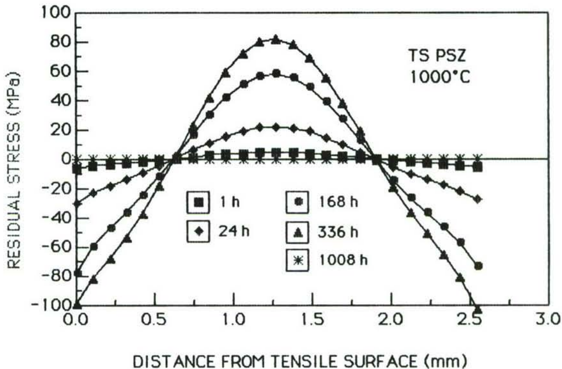
Figure 7. Model predictions indicated the generation of substantial residual stresses within stressed TS flexure specimens.
