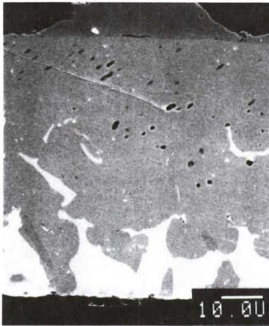
Fig. 4. Electron micrographs of cross sections of zirconia-to-cast-iron bond zones after shear testing at 25 and 400°C. Joints were made with Incusil-15ABA and copper-coated cast iron.
