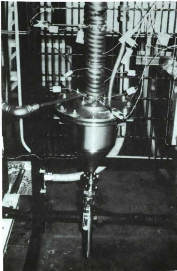
Figure 5. Exit End of Reactor with Simple Thimble Collector and Isolation Valve
