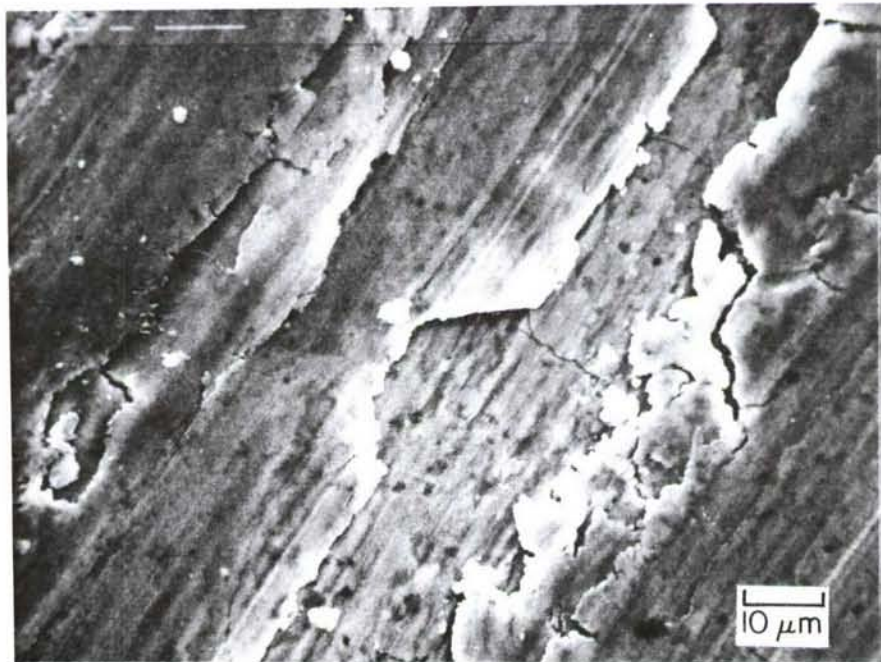
Figure 6. YPSZ wear surface lubricated with \text{MoS}_2 .
