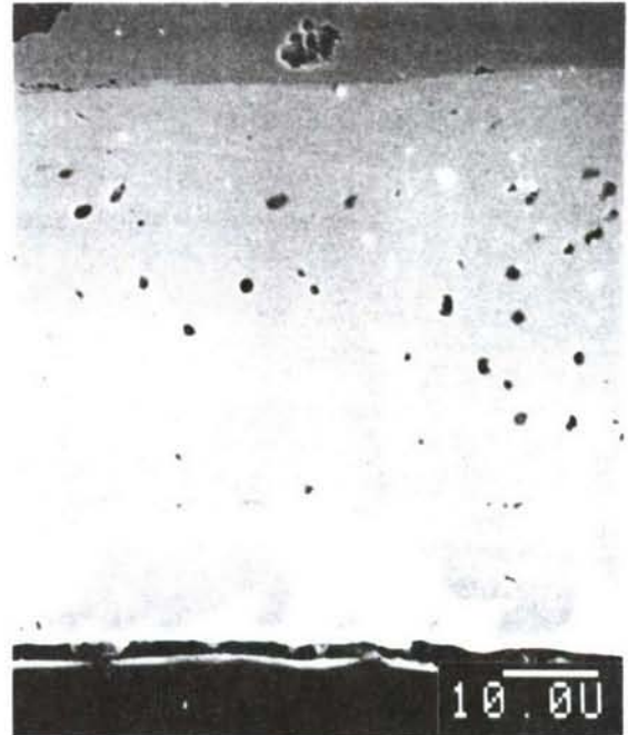
Fig. 4. Electron micrographs of cross sections of zirconia-to-cast-iron bond zones after shear testing at 25 and 400°C. Joints were made with Incusil-15ABA and copper-coated cast iron.
