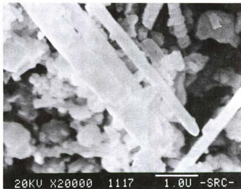
Figures 12A & 12B: Slip cast Si 3 N 4 /ARCO SC-9 SiC whiskers.
