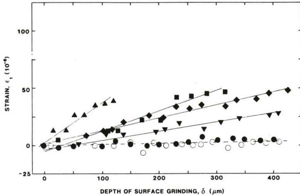
Figure 5. Strain Determination in the Outer Layer of \text{Al}_2\text{O}_3 - 10\text{ZrO}_2 bars (solid circles-inner layer monolithic (code A), open circles-outer layer monolithic (code B), triangles-code C, squares-code D, diamonds-code E, and inverted triangles-code F).
