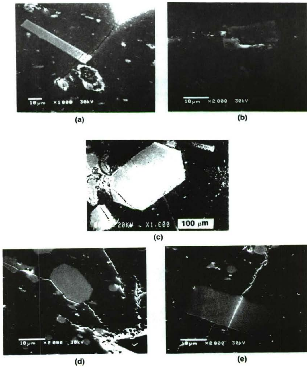
Figure 3: Crack-Dispersoid Interactions in \text{Si}_3\text{N}_4\text{-TiC} Composites (a-c) and \text{Al}_2\text{O}_3\text{-TiC} d,e)
