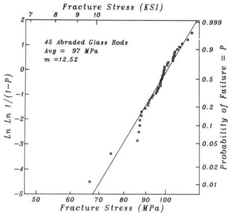
Figure 2. Conventional plot of transformed probability versus log strength with strength data from 45 glass rods.
