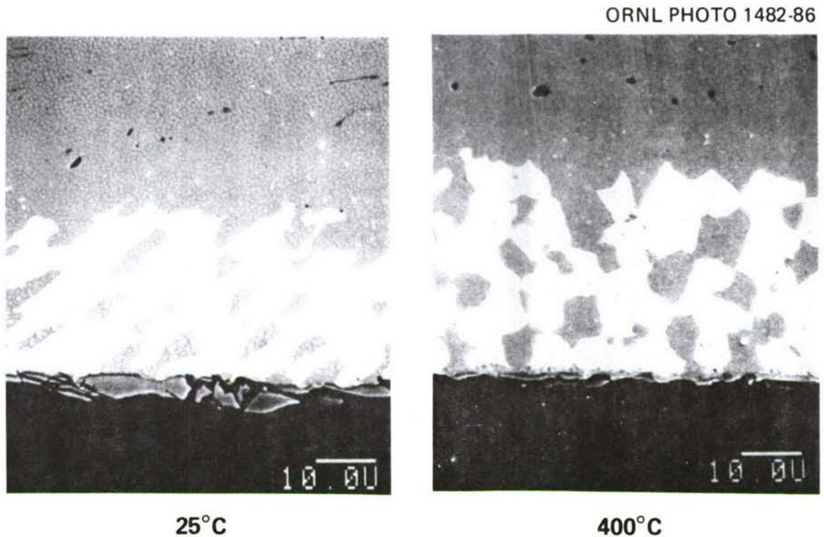
Fig. 2. Electron micrographs of cross sections of zirconia-to-cast-iron bond zones after shear testing at 25 and 400°C. Joints were made by active-substrate brazing.
