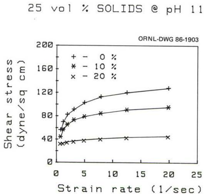
Fig. 1. Adding SiC whiskers to alumina slurries at pH 11 lowered the viscosity of the slurries.
