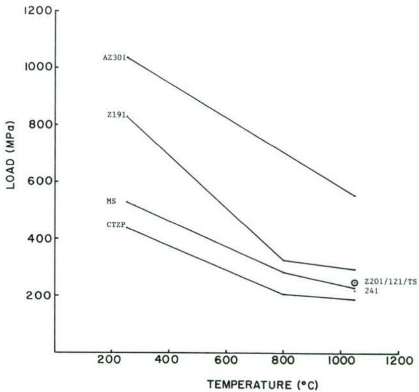
Figure 5. Summary of MOR data in 10% H 2 O at fast loading rates.
