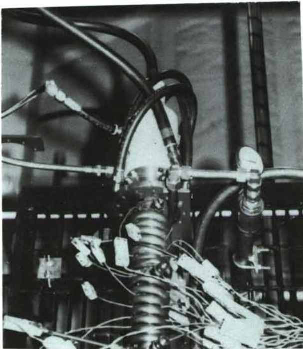
Figure 4. Plasma Torch Atop Water Cooled Reactor
