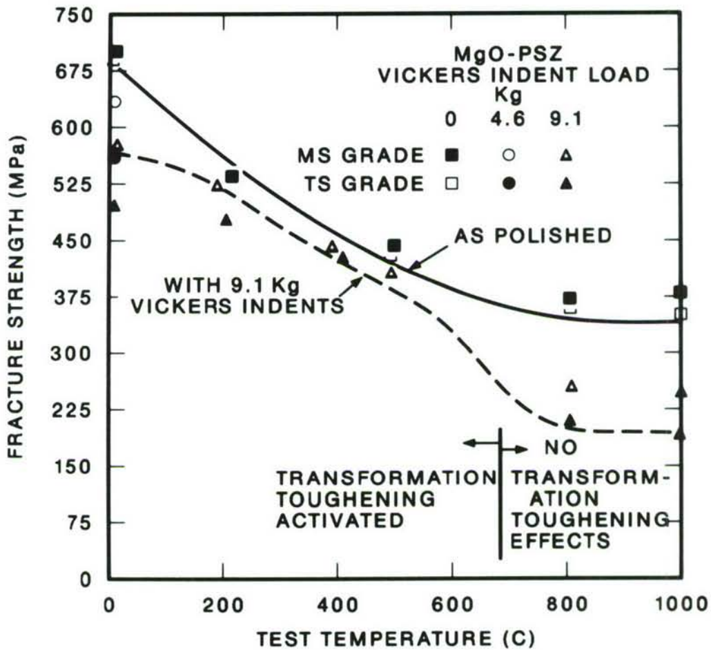
Fig. 3. The fracture strengths of partially stabilized ZrO_2 ceramics are quite insensitive to surface damage. At 500^\circ\text{C} or less, the four-point flexure strengths of MS and TS Grades of PSZ ( K_{IC} \geq 12 \text{ MPa } \sqrt{\text{m}} at 22^\circ\text{C} ) are not substantially lowered when high-load (4.6 and 9.1 kg) Vickers indents are introduced in the tensile surfaces. In this temperature range, the PSZ ceramics exhibit transformation toughening ( K_{IC} \geq 8 \text{ MPa } \sqrt{\text{m}} at \leq 500^\circ\text{C} ). At 800^\circ\text{C} and higher, the strengths are lowered approximately two-fold consistent with the absence of transformation toughening ( K_{IC} \sim 3 \text{ MPa } \sqrt{\text{m}} ).
