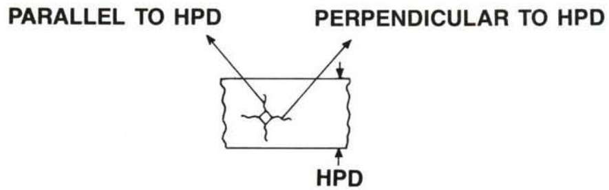
Figure 8: Indentation-Induced Crack Propagation
