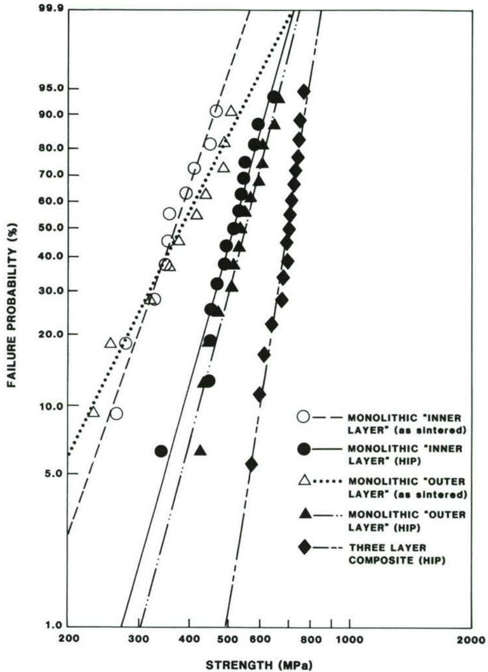
Figure 3. Failure Probabilities of Sintered and Sintered/HIPped Monolithic Materials in Comparison to Sinter/HIPped Three Layer Composite ( d_1=2000 microns). See Table 2 for Weibull moduli.
