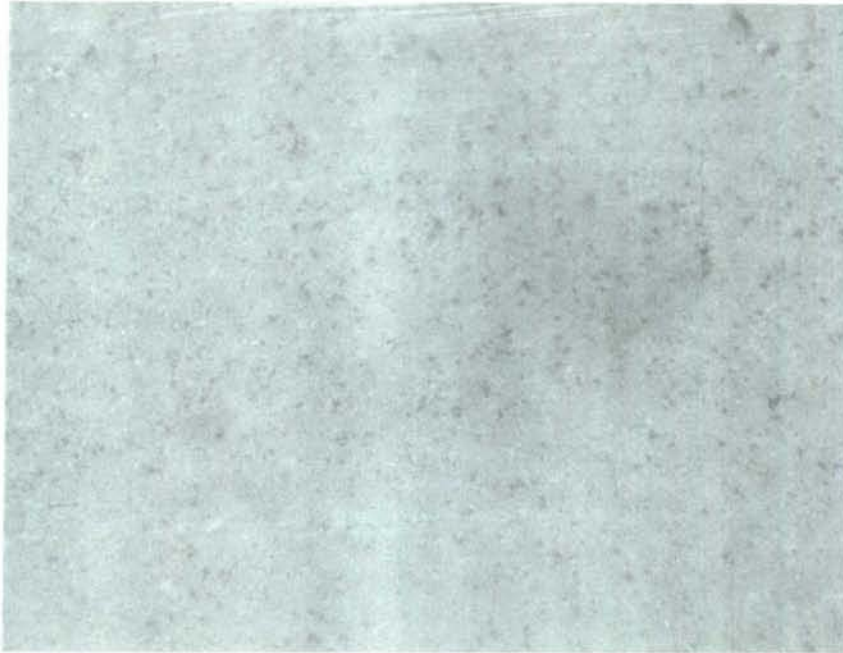
Figure 7A: HIP'ped \text{Si}_3\text{N}_4 /ARCO SC-9 (400X).
