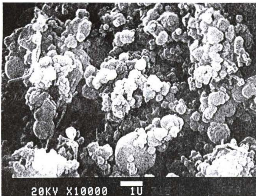
Figure 1. Scanning electron micrograph of powder produced. By x-ray diffraction, the major phase is \alpha - \text{Si}_3\text{N}_4 with \text{Si}_2\text{N}_2\text{O} detected.
