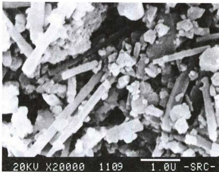
Figures 14A & 14B: Slip cast \text{Si}_3\text{N}_4 /Tateho SCW #1 SiC whiskers.
