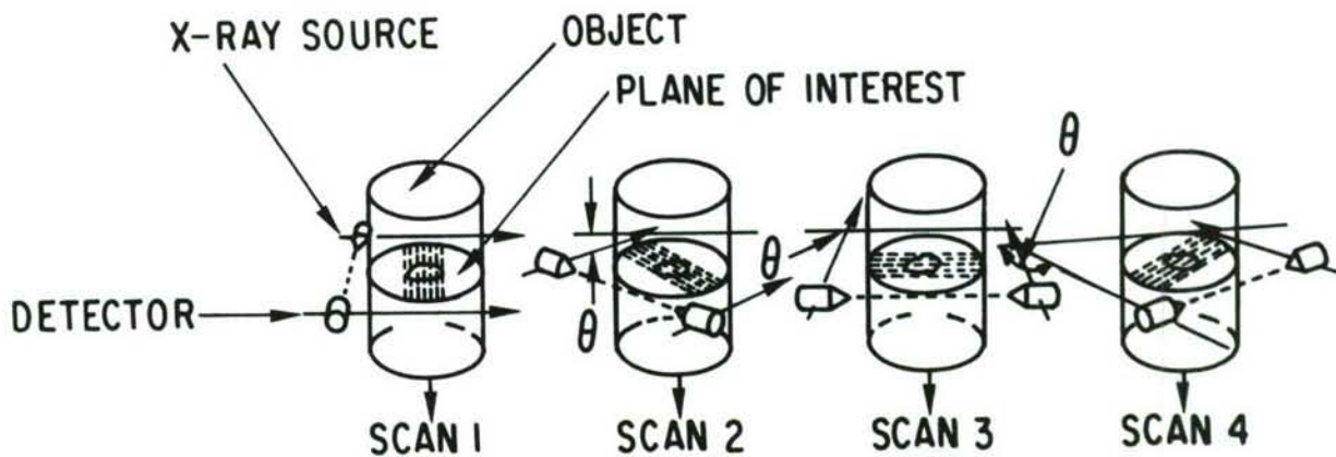
Figure 1. Schematic diagram of the computerized transaxial scanning procedure used to obtain transmission-profile data. The source and detector move synchronously at each \theta position. Four \theta positions are shown.
