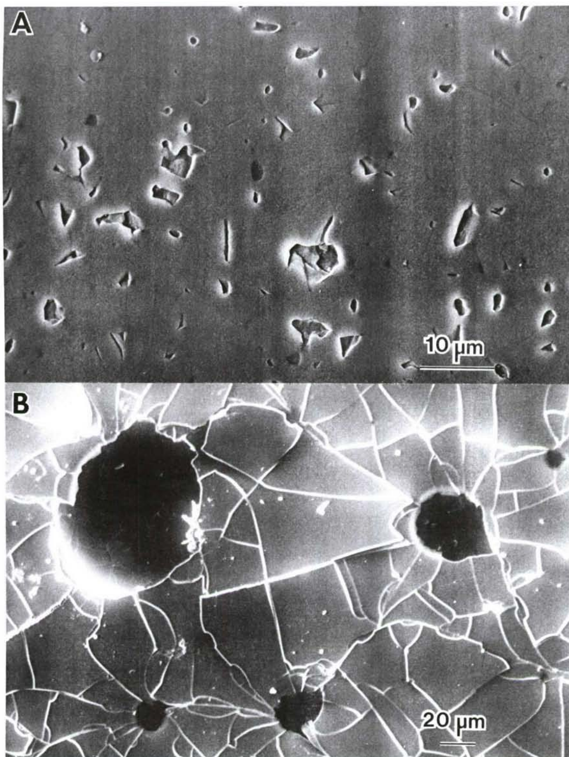
Fig. 1. Sintered alpha SiC after heating 48h at 1000°C. (A) Showing thermal etching on polished surface. (B) Reaction product formed with NaCO 3 on polished surface.
