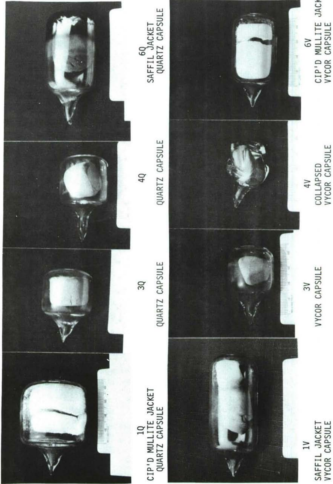
FIGURE 2 GLASS ENCAPSULATED SAMPLES
