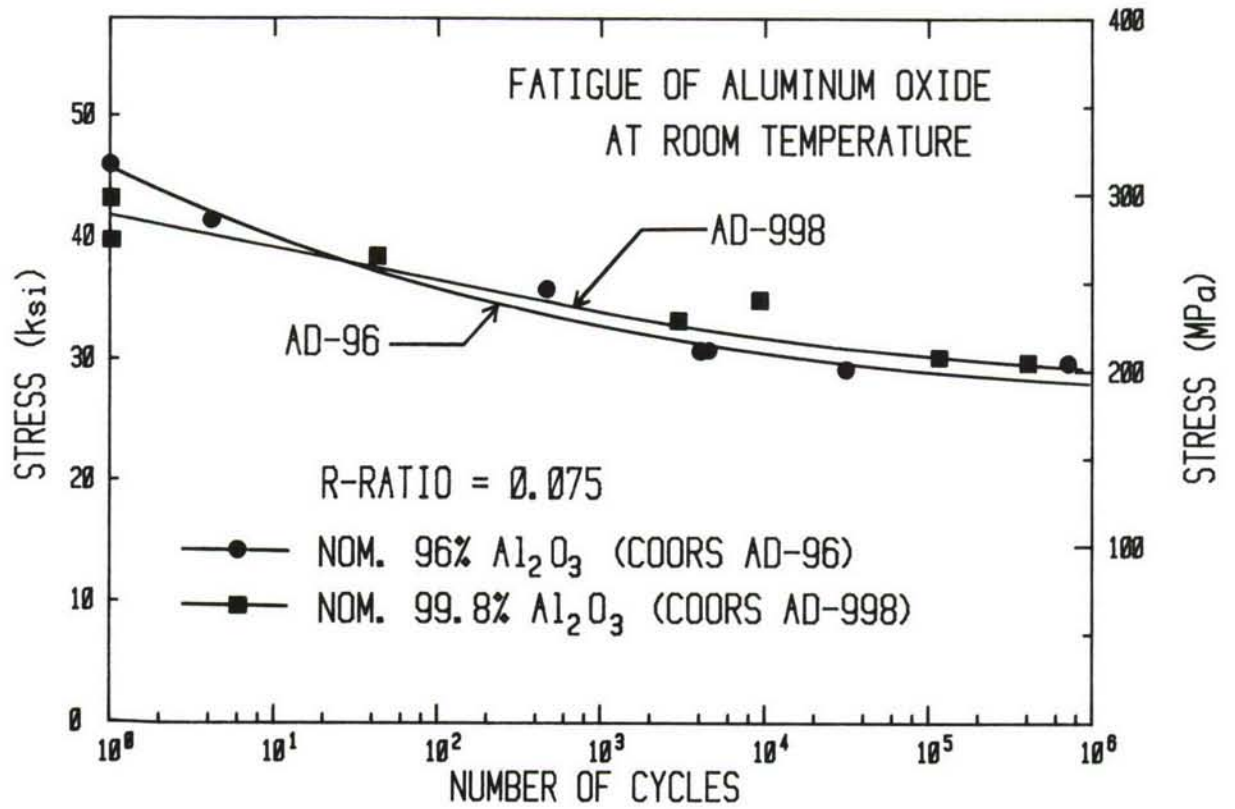
Fig. 5. Comparison between fatigue behavior of Al_2O_3 with 96% purity and that of Al_2O_3 with 99.8% purity, tested at room temperature.
