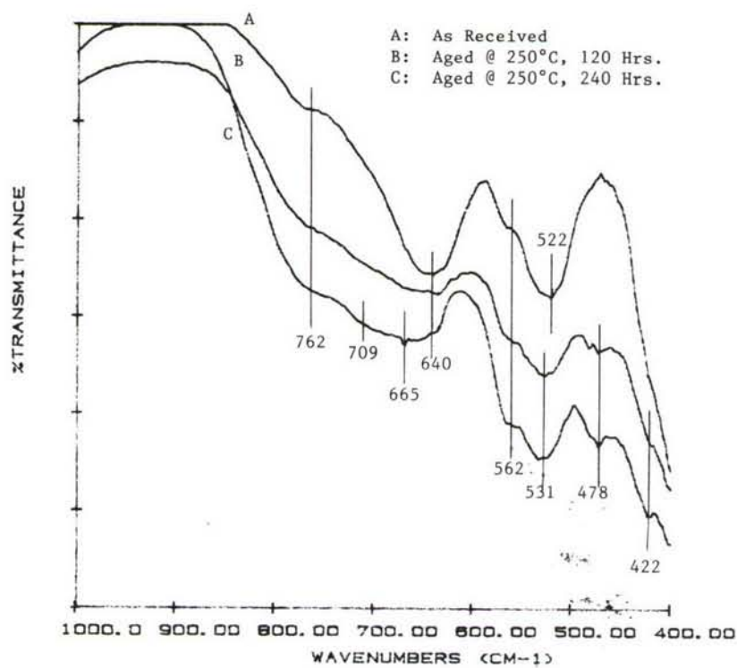
Figure 8. ATR FT-IR spectra for XS241.
