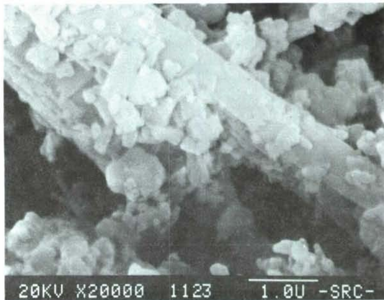
Figures 13A & 13B: Slip cast Si 3 N 4 /coated ARCO SC-9 SiC whiskers.
