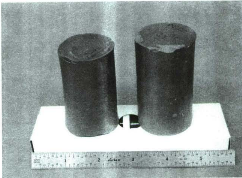
Figure 3: HIP'ped \text{Si}_3\text{N}_4/\text{SiC} whisker samples with Nb encapsulant removed. Left Sample: \text{Si}_3\text{N}_4 /Tateho SCW #1. Right Sample: \text{Si}_3\text{N}_4 /ARCO SC-9.
