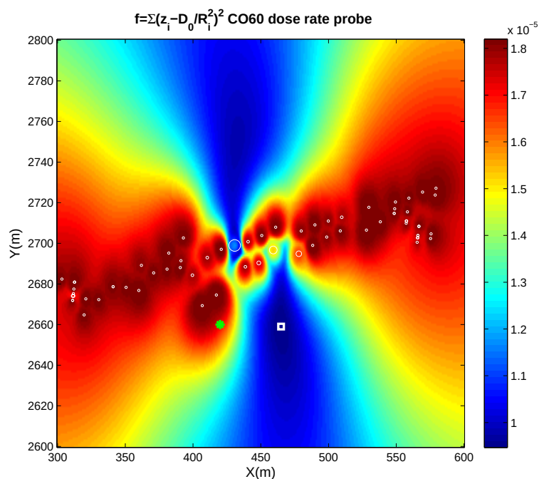
Figure 24: The squared error surface obtained for ^{60}\text{Co} dose rate data. Measurement points (o) and the estimated (□) and true (*) source positions are also shown.
