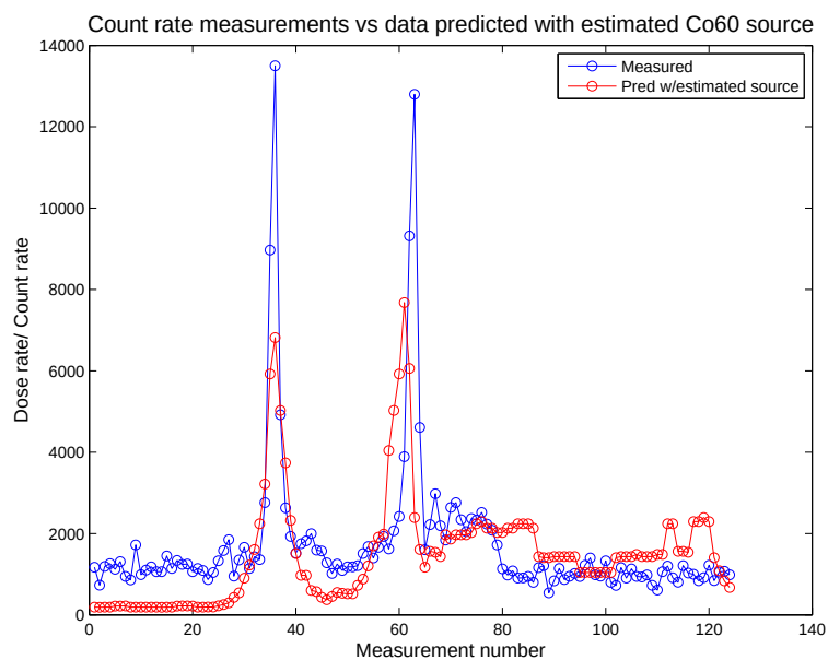
Figure 23: Comparison of ^{60}\text{Co} count rate measurements and prediction based on LS estimation
