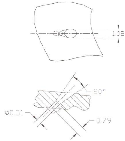
Figure 2. Schematics of the injector geometry, units given in millimeters.
