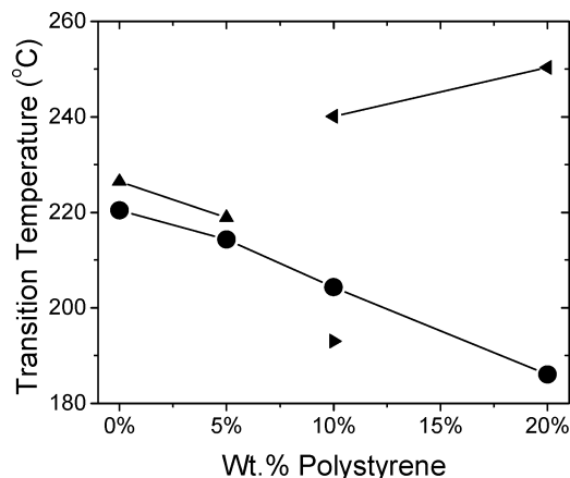
Figure 6. T_{OOT} and T_{ODT} are plotted for both the C-series and L-series. There is an order–order transition in the L-series for the 10 wt % iBu-POSS. All transitions were verified by SAXS. For the C-series, the ● symbol represents the cylindrical–disorder transition. For the L-series, ▲ represents the lamellar–disorder transition, right-tilted ▲ represents the lamellar–cylindrical transition, and left-tilted ▲ represents the cylindrical–disorder transition.
