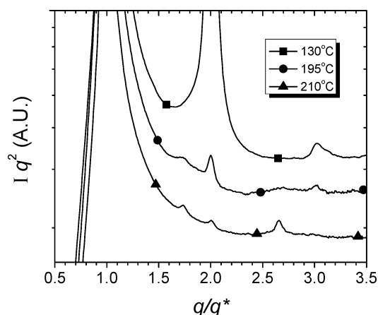
Figure 7. Iq^2 plotted vs q/q^* (where q^* is the q -position of the primary peak) for L-series 10% iBu-POSS at 130 (■), 195 (●), and 210 °C (▲). The morphology is lamellar morphology at 130 °C. A cylindrical morphology is present near the T_{OOT} , 195 °C, and at 210 °C the copolymer is well within the cylindrical morphology temperature range.
