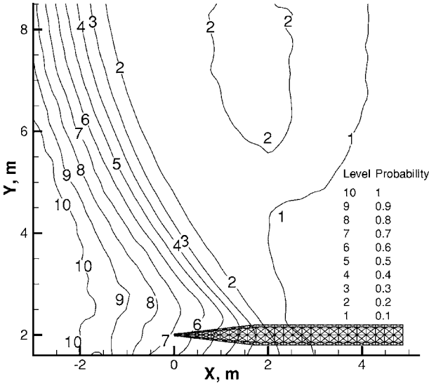
FIG. 2. Reaction probability distribution in the xy plane for O+HCl→OH+Cl using the TCE model (rate constant of Mahmud et al. , Ref. 7) for an altitude of 120 km and a freestream velocity 5 km/s.
