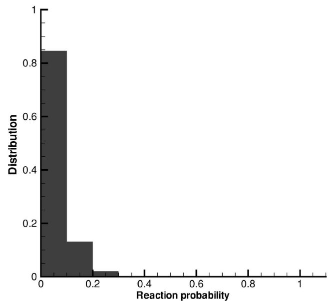
FIG. 22. Reaction probability distribution for O+HCl \rightarrow OH+Cl using the TCE model (the rate of Xie et al. ) for an altitude of 120 km and a freestream velocity 5 km/s.
