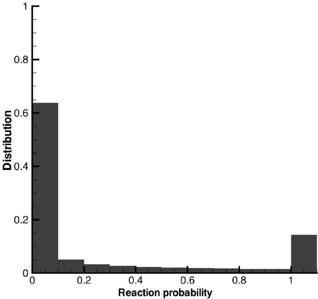
FIG. 3. Reaction probability distribution for O+HCl→OH+Cl using the TCE model (rate constant of Mahmud et al. , Ref. 7) for an altitude of 120 km and a freestream velocity 5 km/s.
