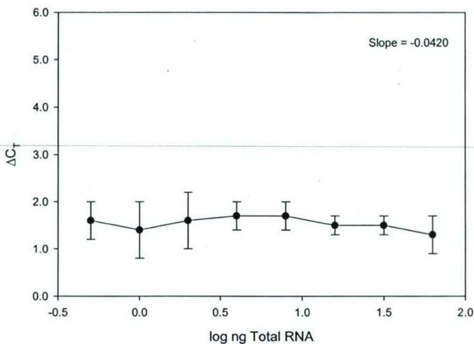
Figure 10. Relative efficiency plot of MT I and GAPDH using additional dilutions of rat liver tissue
