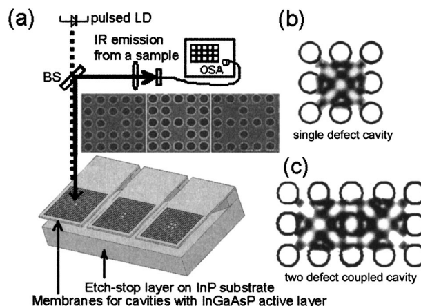
FIG. 1. Two-dimensional photonic crystal slabs with square lattice used in the work: (a) shows drawings of single defect, two-coupled defect, and four-coupled defect cavity membrane structures; (b) and (c) show electric field amplitude profiles in a middle of membrane for single defect and two-coupled defect cavity membrane structures, respectively. One of super-modes is shown for the two-defect coupled cavity.
