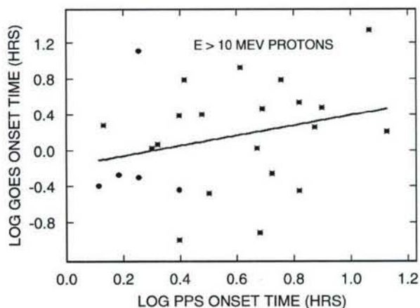
Fig. 3. Comparison of onset times T_{\text{onset}} (from X-ray flare peaks to times when J reaches 10 pfu) for the 25 cases for which PPS predicts a NOAA class SEP event. The least-squares best-fit line is shown, but the PPS predictions are not significantly correlated with the GOES observations.
