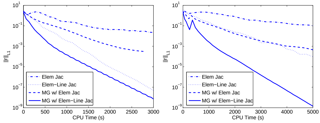
(a) p = 1
