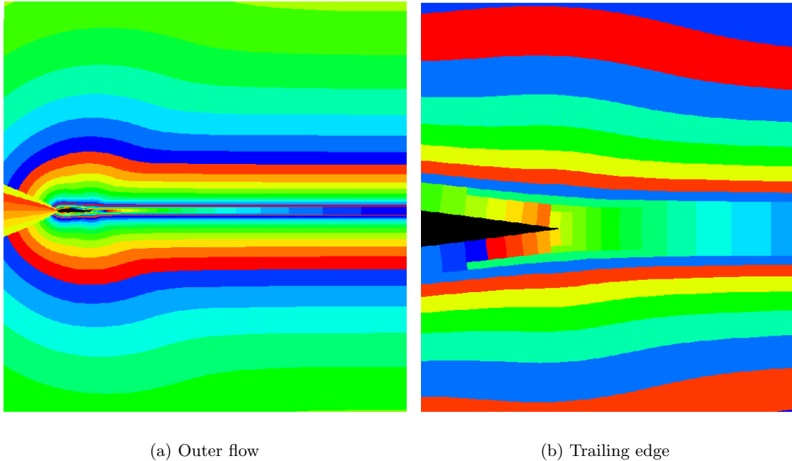
Figure 3-2: Lines formed around NACA 0012 in M = 0.5 , Re = 5000 , \alpha = 0^\circ flow
