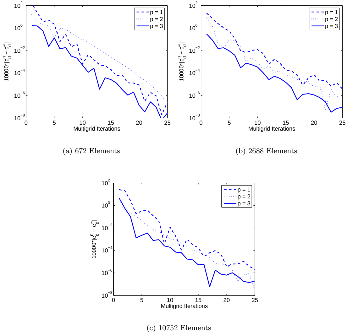
Figure 5-10: Drag convergence history
