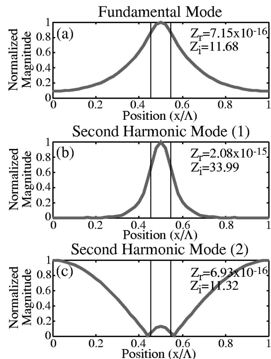
Fig. 3. Properties of the nonevanescient energy-carrying eigenmodes of the nanostructure shown in Fig. 1 for the (a) fundamental and (b), (c) second-harmonic wavelengths computed by using the modified RCWA tool: For each mode the transverse profile in one period of the nanostructure as well as the attenuation coefficient and propagation constant (real and imaginary parts of the corresponding eigenvalue Z respectively) are shown.
