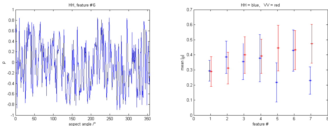
Fig.9 cross correlation coefficient \rho as a function of aspect angle, ft.#6, HH Fig.10 |\rho| averaged over 360^{\circ} for all 7 features, HH=blue, VV=red
