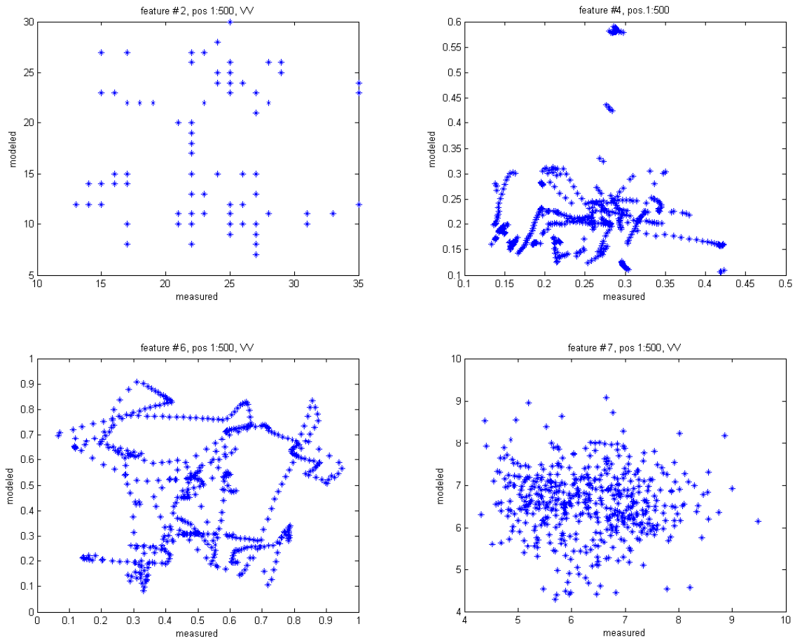
Fig.8 scatter plots measured vs. modeled data for features 2, 4, 6 and 7. Aspect angle 0^{\circ} - 15^{\circ} , VV polarisation
