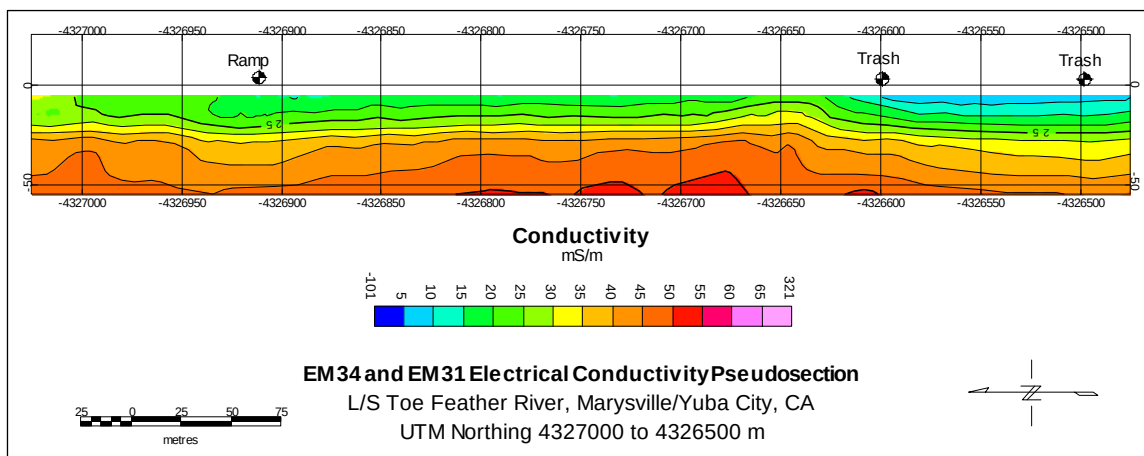
Figure C3. EM31 and EM34 electrical conductivity pseudosection, UTM Northing 4327000 to 4326500 m.
