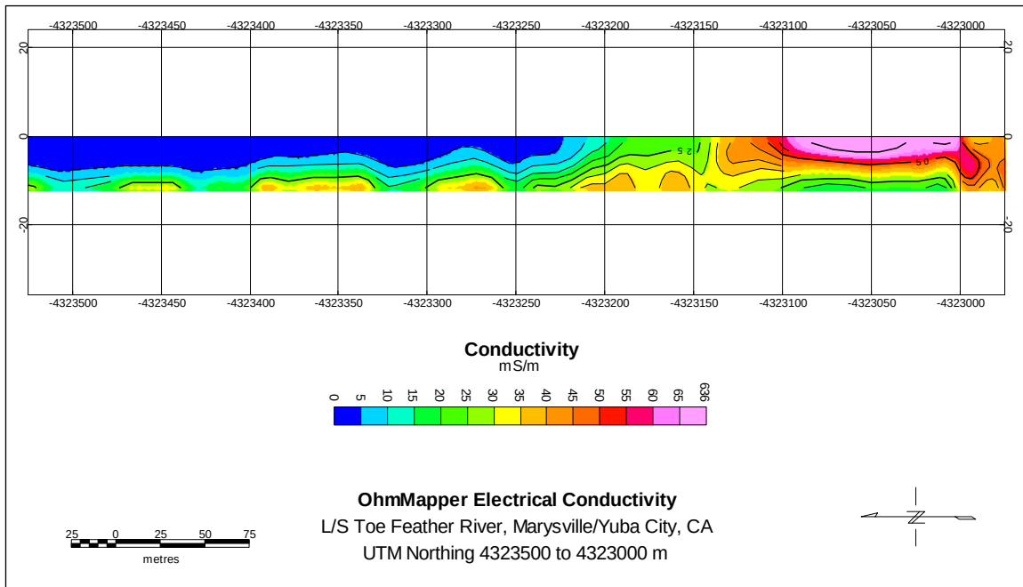
Figure E10. OhmMapper electrical conductivity depth section, UTM Northing 4323500 to 4323000 m.
