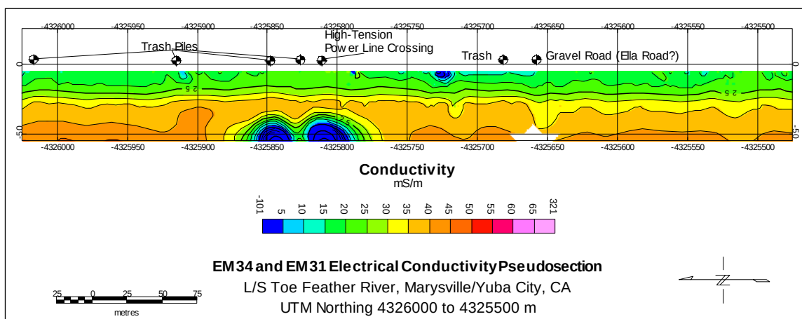
Figure C5. EM31 and EM34 electrical conductivity pseudosection, UTM Northing 4326000 to 4325500 m.
