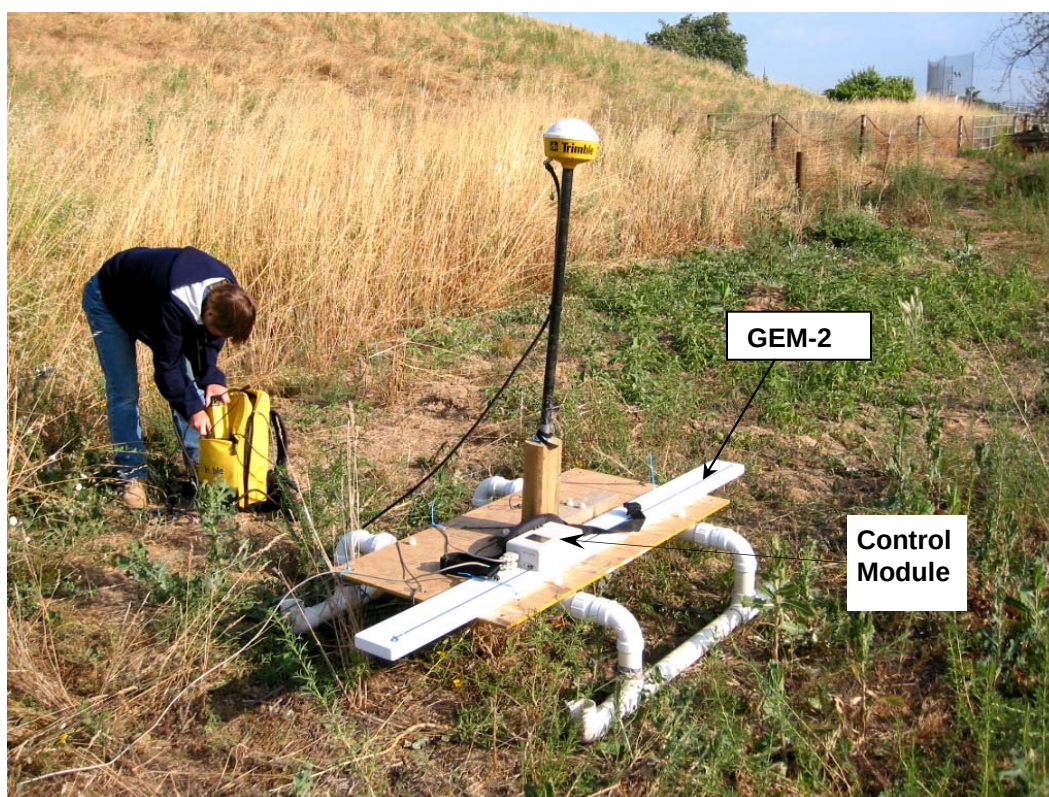
Figure 4. A sled-mounted Geophex GEM-2 multi-frequency EM induction instrument being prepared for surveying.
