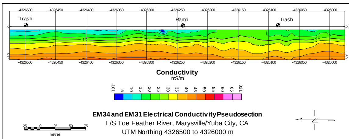
Figure C4. EM31 and EM34 electrical conductivity pseudosection, UTM Northing 4326500 to 4326000 m.
