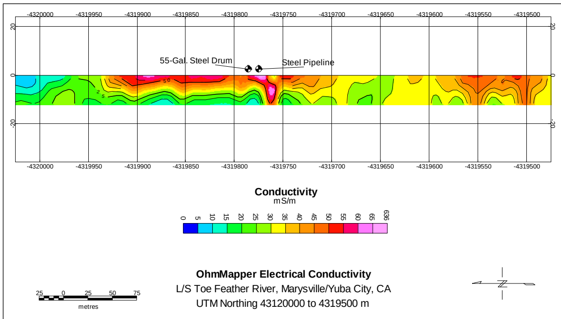
Figure E17. OhmMapper electrical conductivity depth section, UTM Northing 4320000 to 4319500 m.
