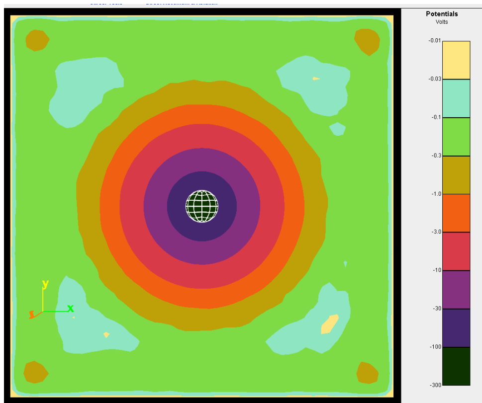
Figure 6. Potentials at 25 microseconds corresponding to Figure 5.
