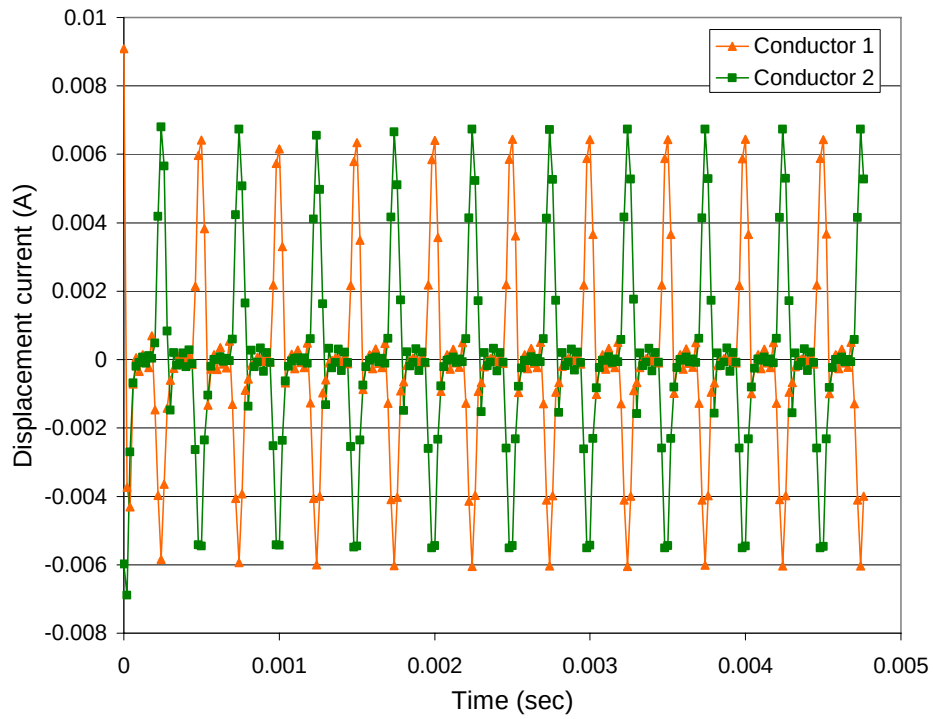
Figure 43. Displacement current for Case 3.
