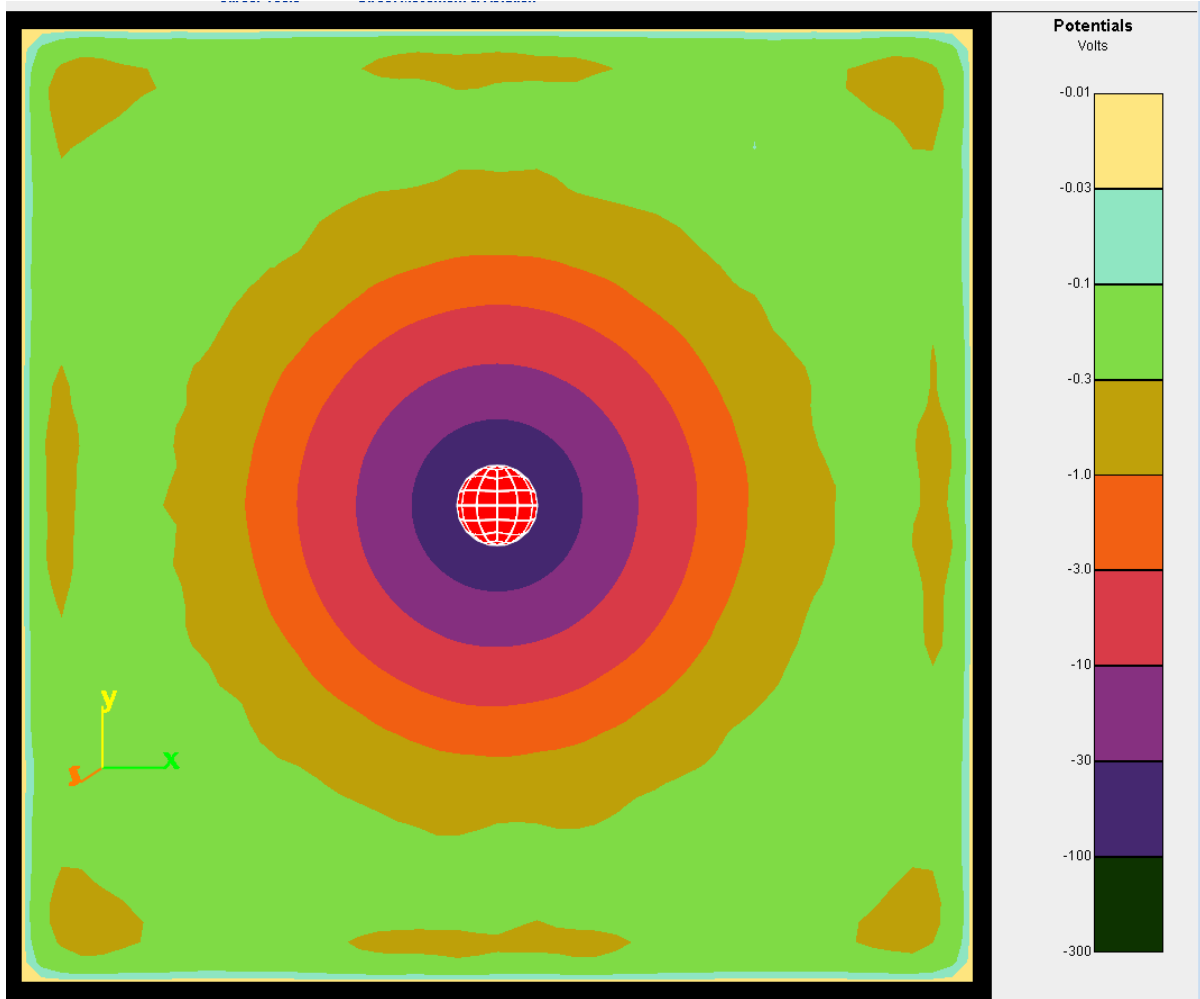
Figure 4. Potentials at 25 microseconds corresponding to Figure 3.
