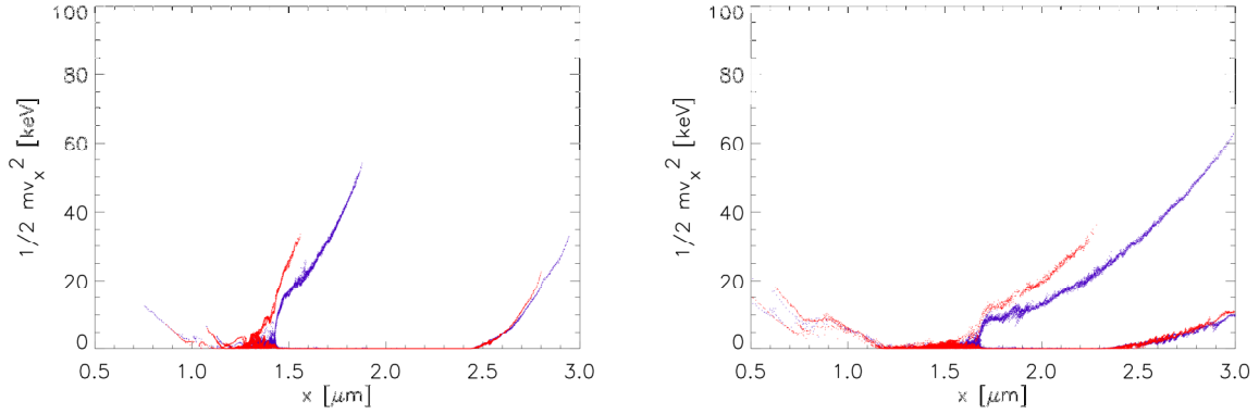
Figure 5: Spatial energy distribution of the D (blue) and T (red) population after 0.48ps (left) and 0.96ps (right) for a laser intensity of I=1.8 \cdot 10^{17} \text{ W/cm}^2 .
