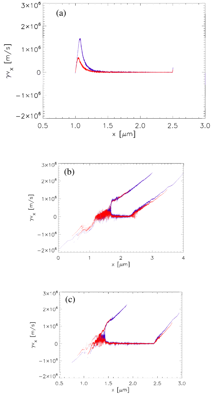
Figure 4: Phase space projections of the D (blue) and T (red) ions at different times: (a)- 96fs, (b)-0.48ps and (c)- 0.96ps.
