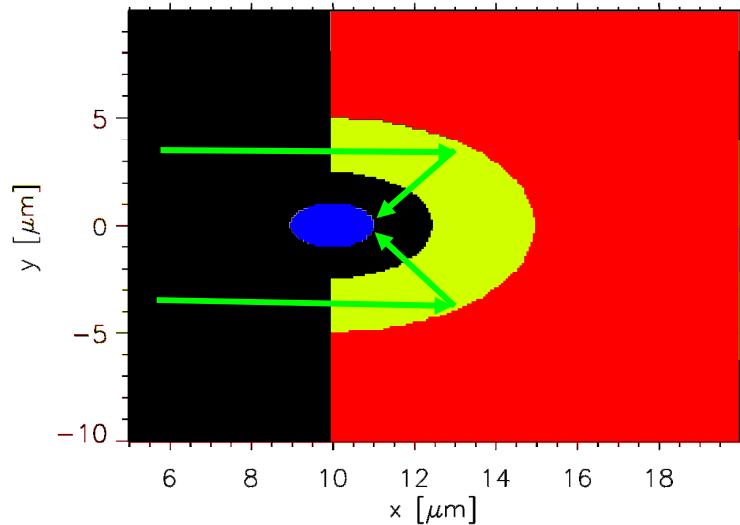
Figure 13: Setup of shaped target configuration: A high density shaped tin target (red) is coated with an under-dense deuterium film (yellow) with a Tritium ball (blue) suspended in the center of spherical mirror. The Tritium ball has a diameter of 2\text{ }\mu\text{m} , the Deuterium coating has a thickness of 2.5\text{ }\mu\text{m} . The cavity/mirror radius is 5\text{ }\mu\text{m} . The laser pulse enters from the left, is reflected off the spherical mirror and gets focused in the center of the mirror.
