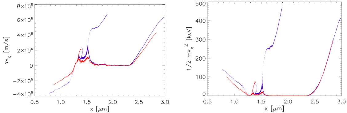
Figure 6: Phase space projection (left) and ion energy (right) for the interaction of a 60 fs, 2.6 \cdot 10^{17} \text{ W/cm}^2 laser pulse with a D-T plasma.
