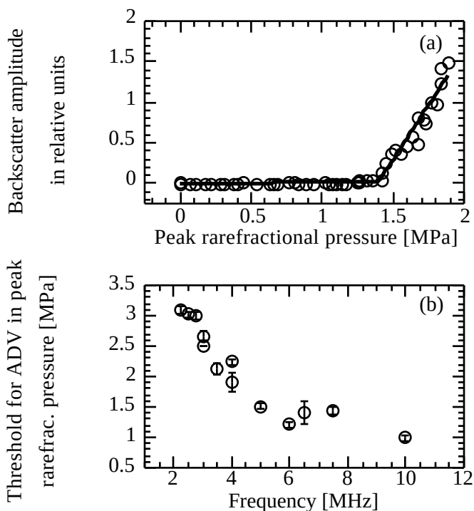
Figure 2: (a) At 7.5 MHz the threshold for acoustic vaporization of droplets is approximately 1.5 MPa PRP. At lower pressures droplets rarely, if ever, boil into gas bubbles. Therefore ultrasonic images of the area to be treated can be taken at pressures below 1.5 MPa PRP. The threshold for ADV is a function of frequency; it rises with decreasing frequency (b).
