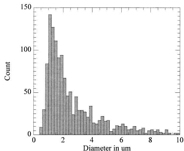
Fig. 4. Size distribution for DDFP droplets made with 1 mg albumin per mL. The mean size is 1.5 \mu\text{m} radius. The total number of droplets was 1332 for an approximately 3 \times 10^{-5} \text{ mL} sample volume, corresponding to a concentration of 4.82 \times 10^7 droplets per mL.
