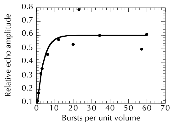
Fig. 1: The efficiency of ADV is evaluated by fitting the relative echo amplitude to the number of bursts each unit volume of droplets is exposed to.
