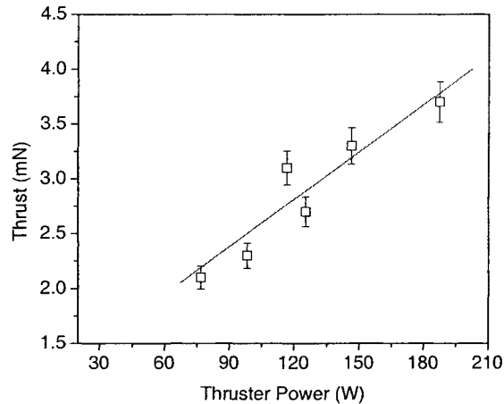
FIG. 3. Thrust performance over range of discharge power.
