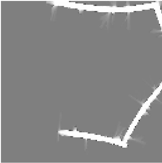
Figure 3.6a: Naïve map
