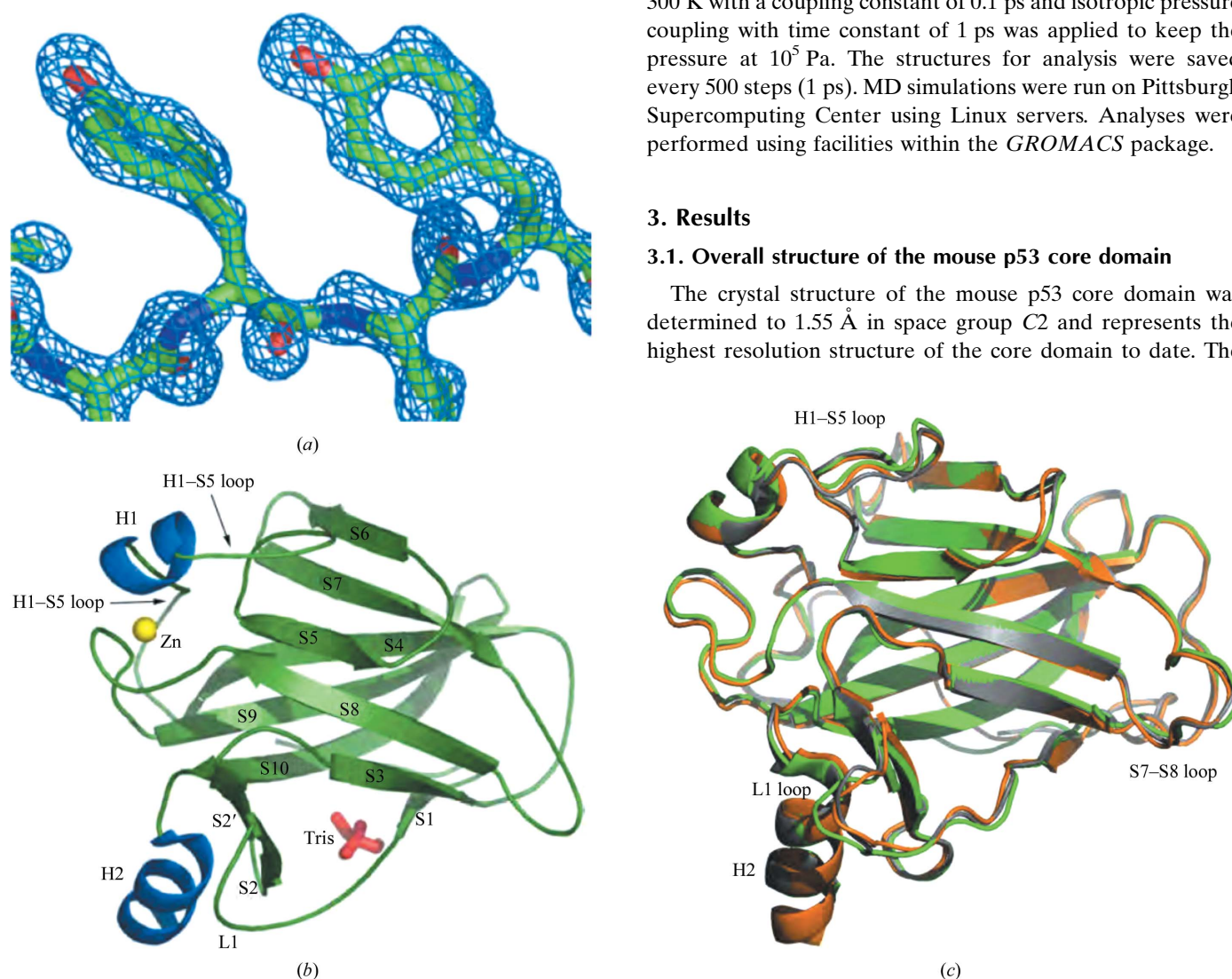
Figure 1 Overall structure of the mouse p53 core domain. (a) Representative F_o - F_c OMIT electron-density map of residues 231–233 contoured at 3.5\sigma . (b) Overall structure of the mouse p53 core domain solved to 1.55 Å resolution. The Zn atom is shown as a yellow sphere and a molecule of Tris is shown in red. (c) Overlay of the mouse core domain solved at 1.55 Å resolution in space group C2 (HR, green), the mouse p53 core domain solved at 2.7 Å in space group C222 1 (PDB code 1hu8, grey) and the human p53 core domain unbound to DNA (PDB code 1tsr; orange)
