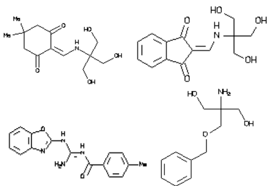
Figure 1. Structure of 4 Tris like compounds that showed favorable p53 docking properties.
