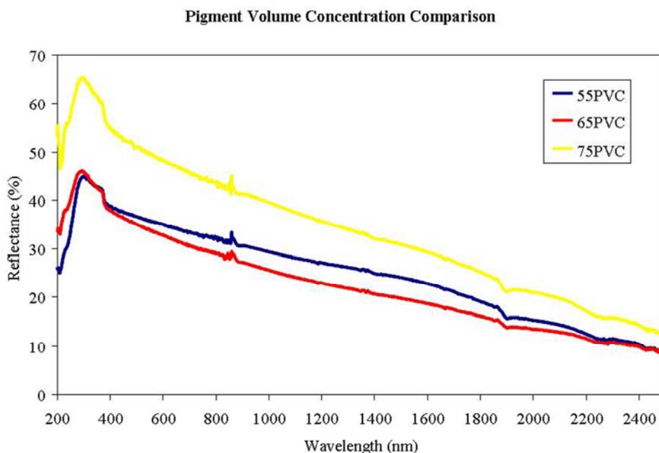
Figure 10. Reflectance of “virtual” pigment films with various pigment volume concentrations of hollow silica microspheres.
