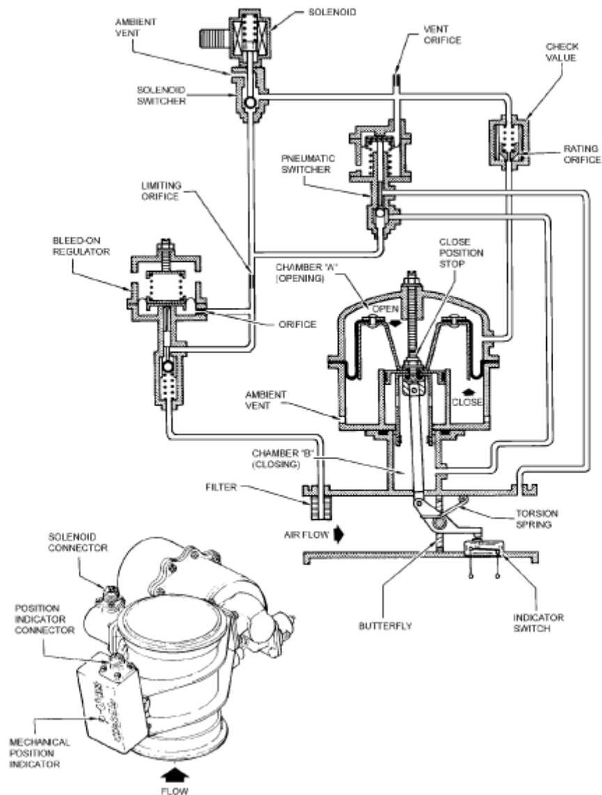
Figure 2-16: Starter Air Regulating Valve from Reference 12
