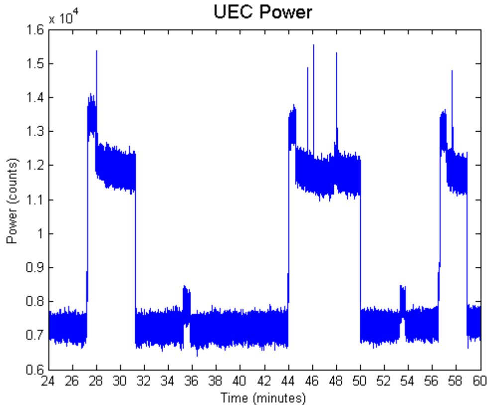
Figure 3-8: Unfiltered power data from the UEC NILM
