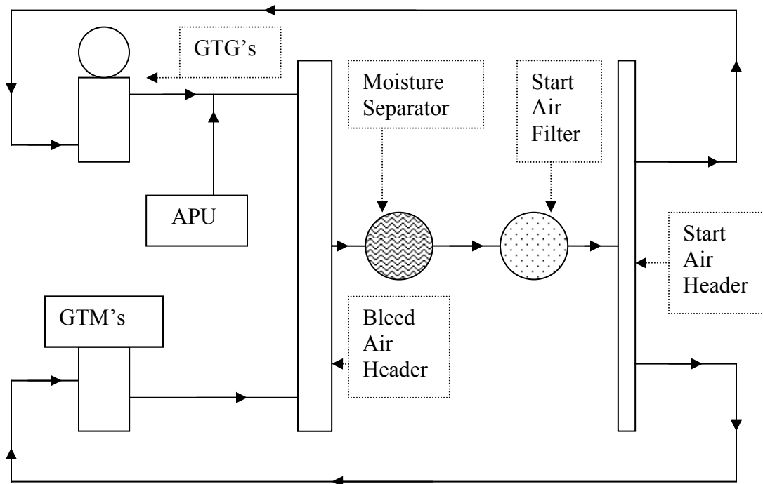
Figure 2-8: Bleed and Starter Air Block Diagram
