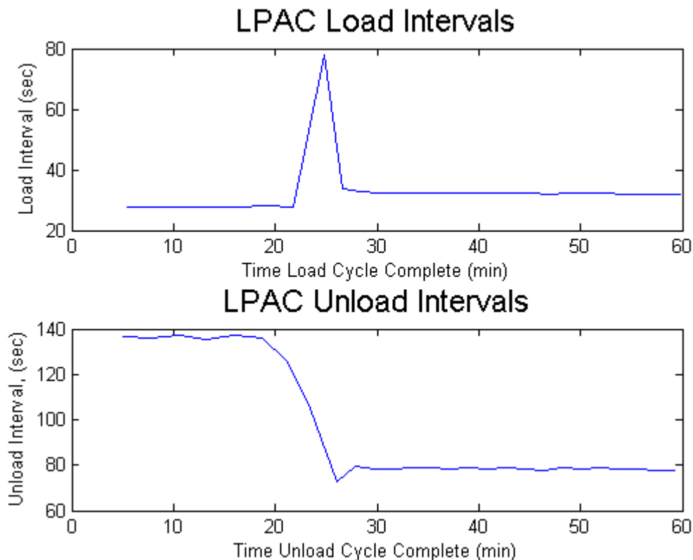
Figure 3-5: Loaded and unloaded times before, during, and after an air start of Unit 9130 (#2 Gas Turbine Generator) between 7:00 a.m. and 8:00 a.m. on April 22, 2005.
