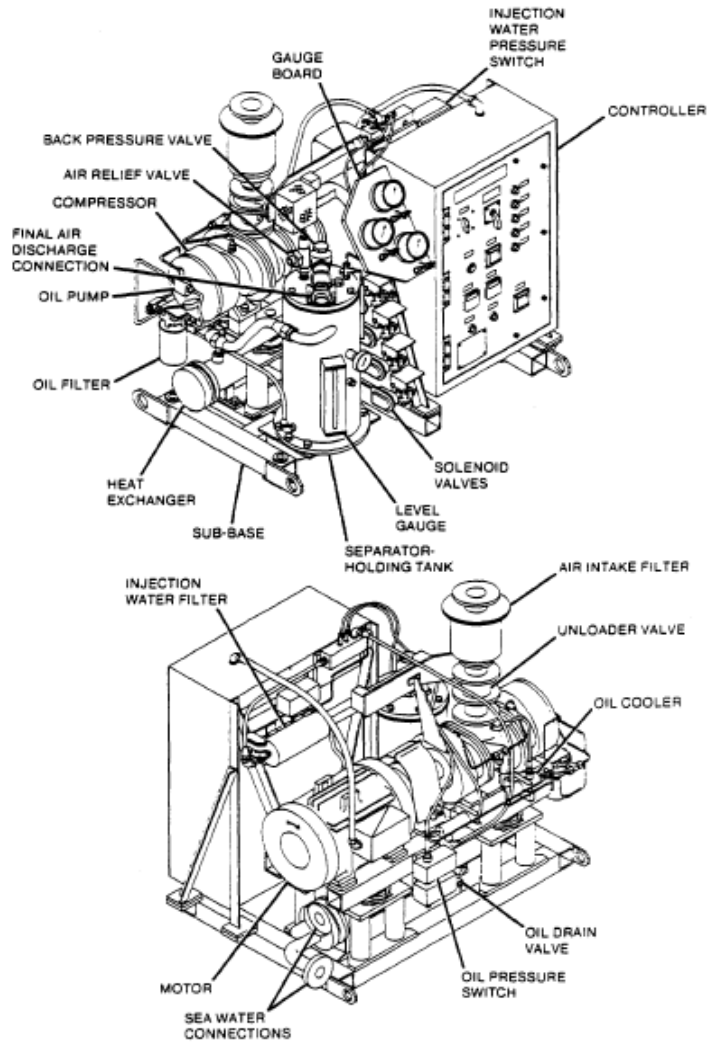
Figure 2-11: LBES Low Pressure Air Compressor from Reference 15
