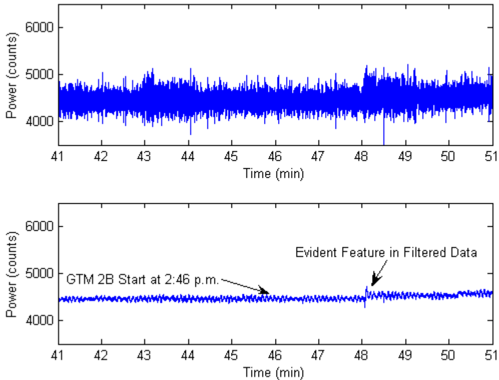
Figure 3-7: Unfiltered (top) and filtered (bottom) power data from the fuel oil pump NILM. GTM 2B was started at 2:46 p.m. per operator logs. A noticeable feature appears in the filtered data two minutes afterwards.
