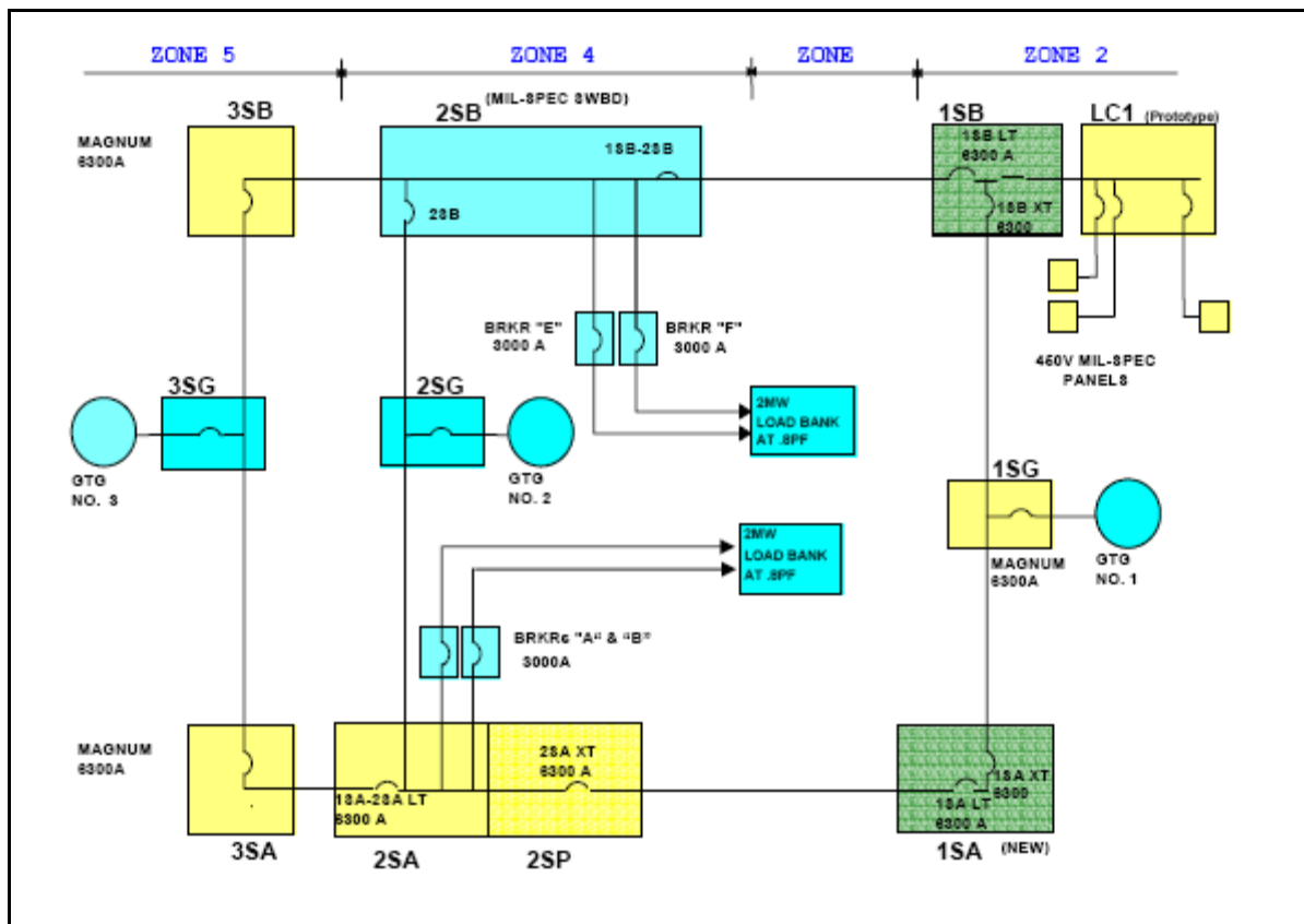
Figure 2-14: LBES Electrical Distribution System
