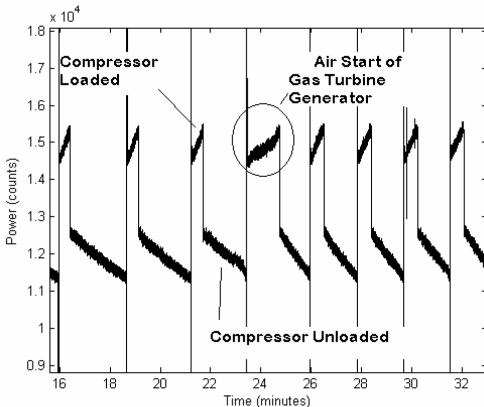
Figure 3-4: Plot of the real power drawn by the LPAC before, during, and after an air start of Unit 9130 (#2 Gas Turbine Generator). The units of real power are shown here to be counts, and they reflect the scale factors introduced by our instrumentation. The power can be converted into Watts by determining the appropriate multiplicative scale factor to apply to the data.
