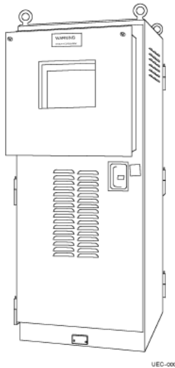
Figure 2-7: Universal Engine Controller (Exterior View) from Reference 13
