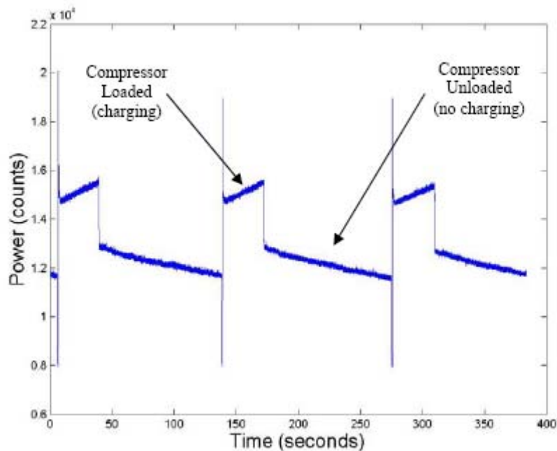
Figure 3-3: LPAC in Automatic 125 PSIG Operation
