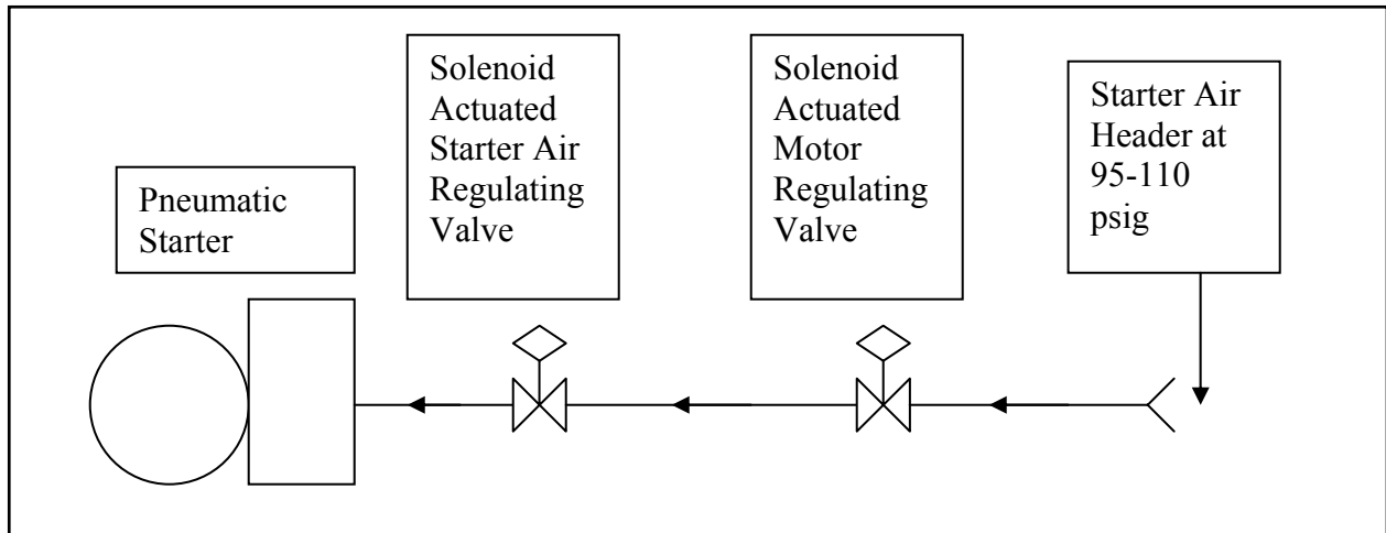
Figure 2-17: Starter and Motor Regulating Valve Locations
