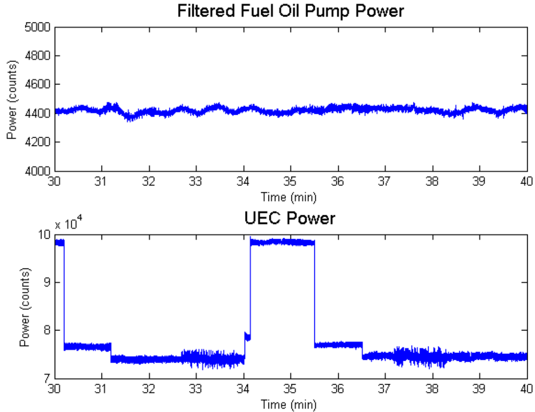
Figure 5-1: Filtered Fuel Oil pump power and UEC power during a failed GTM 2B start at approximately 10:30 a.m. on April 25, 2006. The Fuel Oil pump power remains unaltered during the failed start. This may indicate a fault in the Fuel Oil system vice the UEC, SCU, etc.
