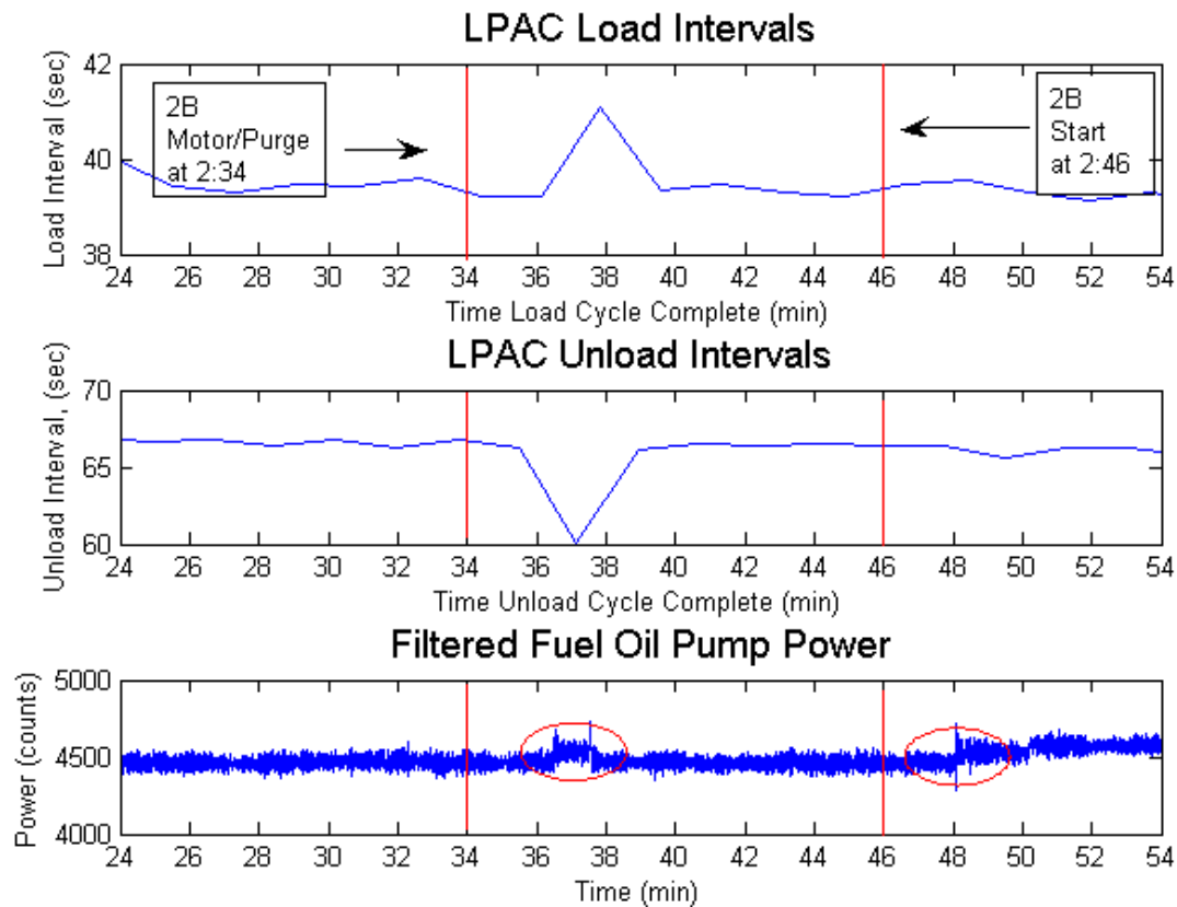
Figure 4-1: Combined NILM data from LPAC Load-Unload plot and filtered Fuel Oil pump data for a GTM start and Motor/Purge. The data was recorded between 2:00 and 3:00 p.m. on April 18, 2005. The GTM start impacts the Fuel Oil pump behavior, but not the LPAC.
