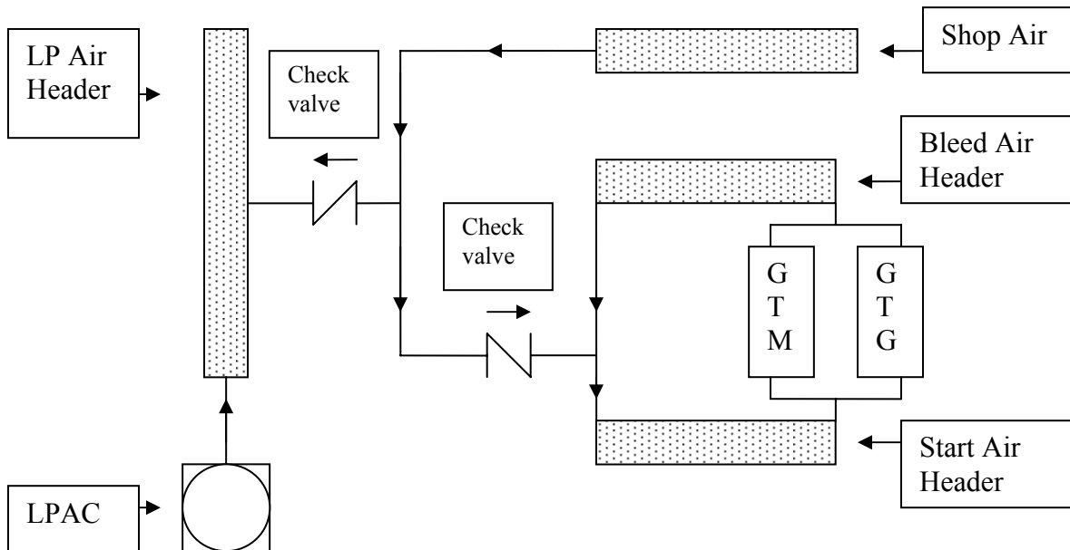
Figure 2-10: Low Pressure Air system relationships at the LBES. Shop air typically operates at 95-110 psig, and the LPAC maintains the LP Air header at 110-125 psig.
