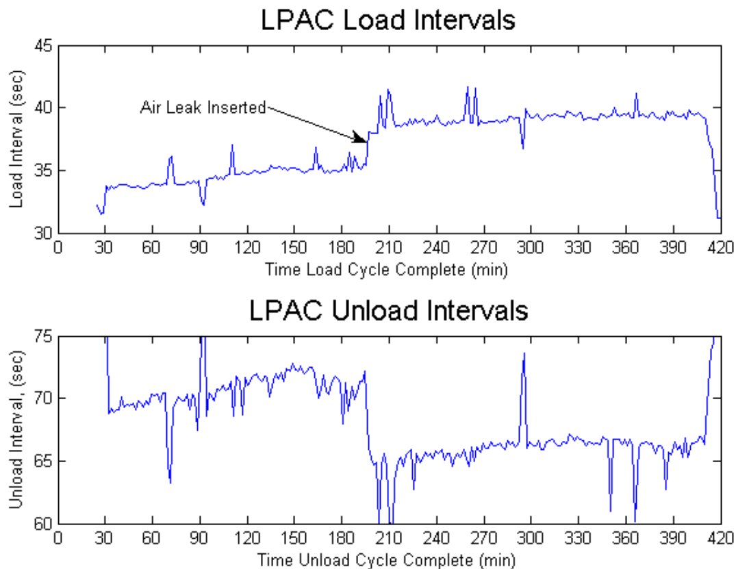
Figure 4-12: LPAC Load-Unload data for April 18, 2005. All hour long snapshots have been concatenated and then passed through the Load-Unload Script. The exact time of the air leak insertion was recorded during previous research.
