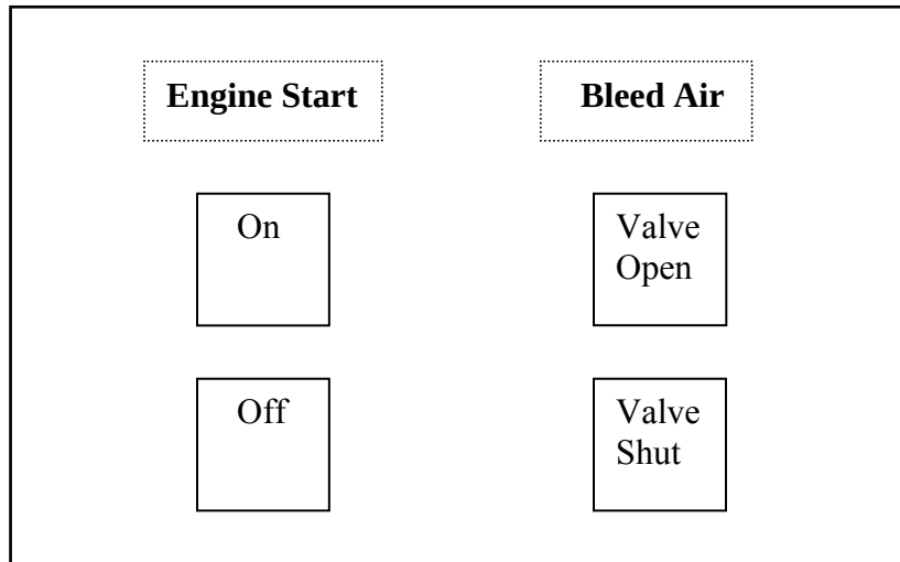
Figure 2-15: Simplified GTG Controls at the EPCP
