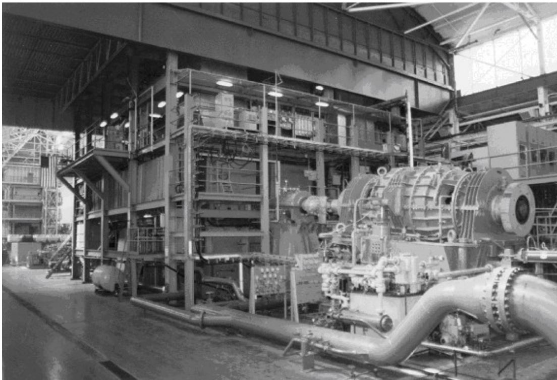
Figure 2-2: DDG-51 Land Based Engineering Site (LBES)
