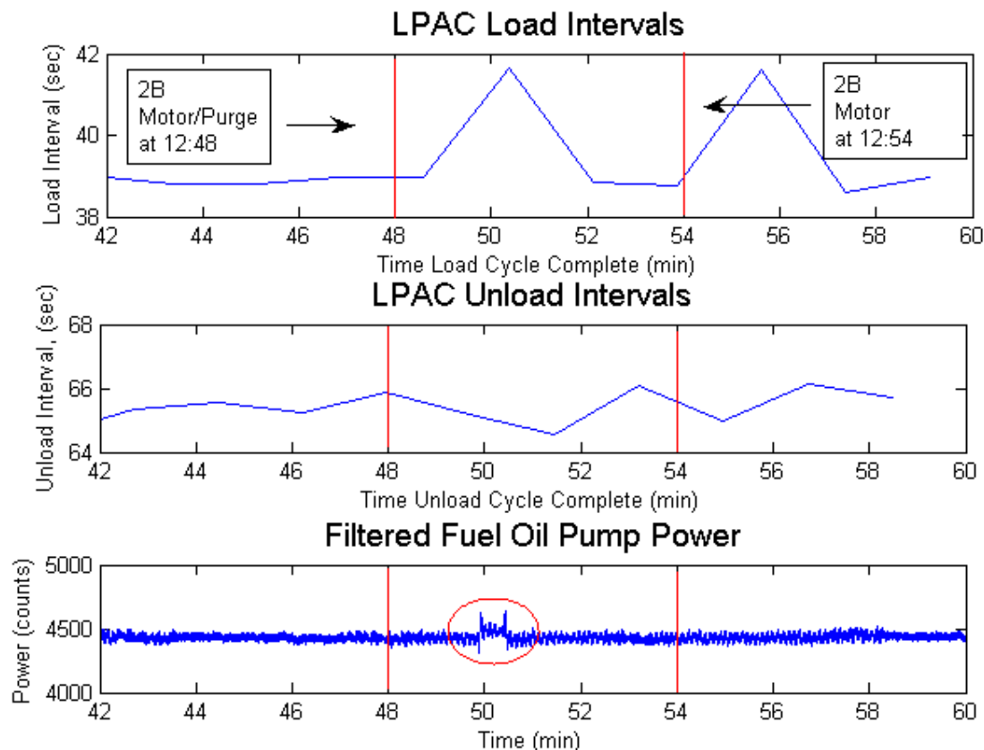
Figure 4-6: A motor/purge event is contrasted with a motor event. These events occurred between 12:00 and 1:00 p.m. on April 18, 2005. Both motoring events affect the LPAC via the Motor Regulating valve, but only the motor/purge affects the fuel oil system, and thus the Fuel Oil pump.
