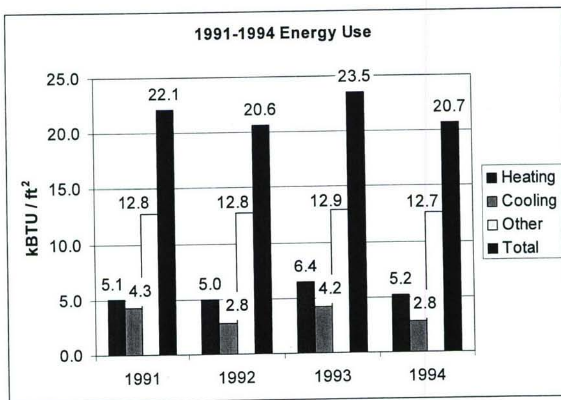
Figure 3 – Actual Energy Use of Plumblee Home
