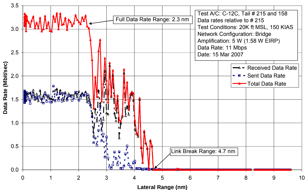
Figure E-1. Example data rate collected during Varying Range FTT (30 deg Outbound)
