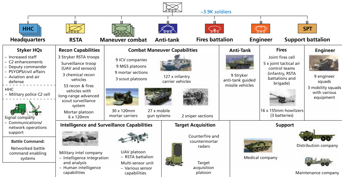
Figure C.2 Design of the Army Stryker Brigade Combat Team
