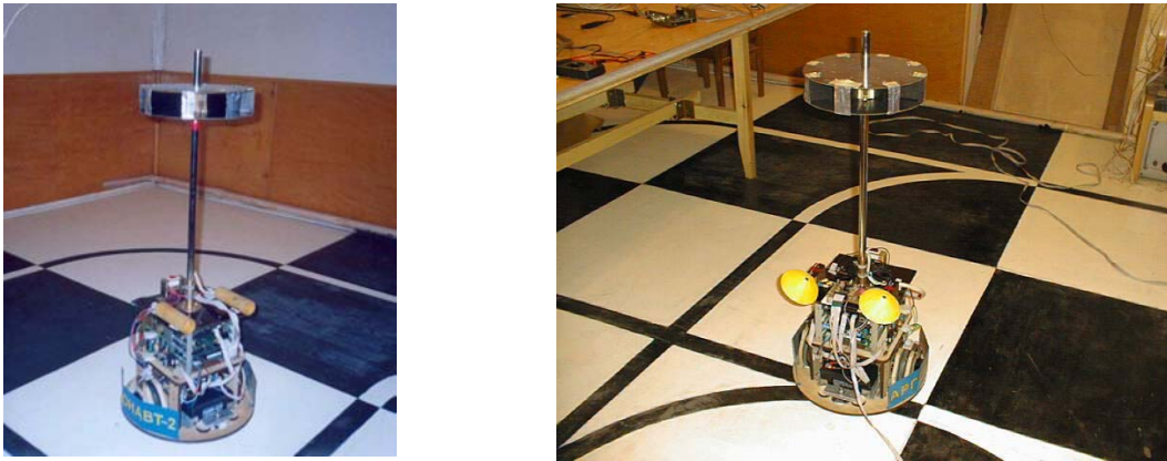
Figure 1: The “Argonaut-2” Mobile Robot Equipped with Audition Sensors.
