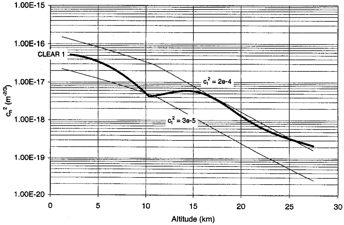
Figure 3: CLEAR 1 Profile and curves for two constant values of C_T^2 .
