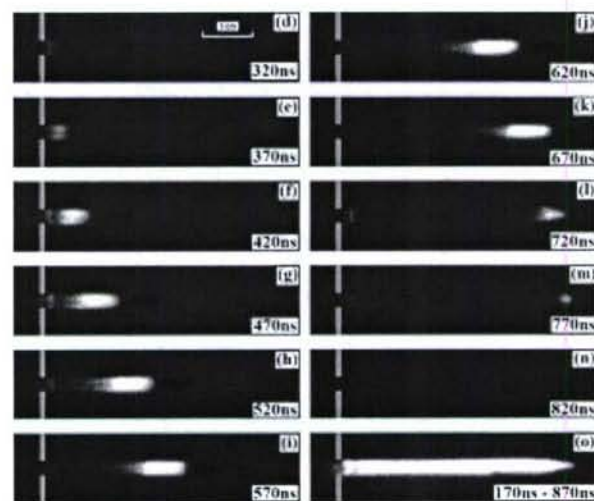
Fig. 28 ICCD pictures of the plasma plume
