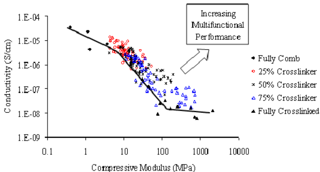
Figure 6. Room temperature ion conductivity vs. stiffness for vinyl ester copolymer electrolytes.
