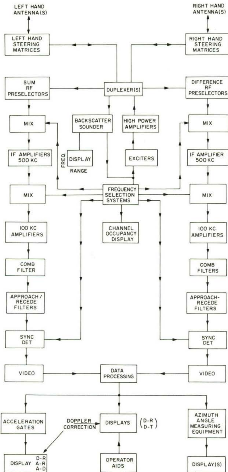
Fig. 8 - Block diagram of generalized system
