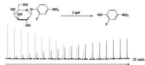
Figure 2. Conversion of OFNPNG to OFPNP by stably transfected PC3- lacZ cells. Stacked plot series showing the conversion of OFNPNG ( 2.9 mg; 9 mmol) by PC3- lacZ prostate cancer cells ( 2 \times 10^7 in PBS, pH 7.4 at 37^\circ\text{C} ) to the aglycone OFPNP, which resonates \sim 5 ppm upfield of the substrate (OFNPNG, gray traces, OFPNP black traces). Sequential spectra were acquired in 102 s each over a period of 31 min.
