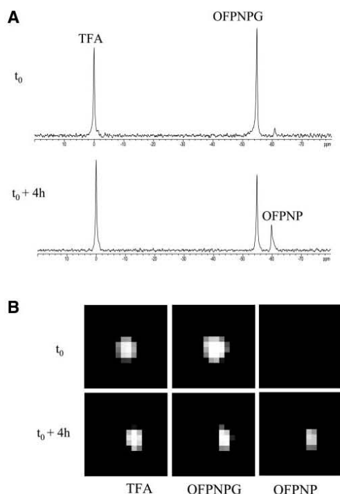
Figure 3. Conversion of OFPNPG to OFPNP by PC3- lacZ cells detected using ^{19}\text{F} -CSI at 4.7 T. PC3- lacZ cells ( 10^7 ) were added to a 1 cm diameter vial containing OFPNPG (15.6 mg; 48 mmol (70 mM) and imaged over a period of 4 h at the ambient temperature of the magnet bore ( \sim 16^\circ\text{C} ): field of view = 30 \times 30 mm, spectral width = 70 ppm, one slice with thickness = 10 mm, data matrix = 16 \times 16 voxels, TR/TE = 1000/12 ms, 4 averages. A) Bulk spectra and B) chemical shift images each acquired in 5 min.
