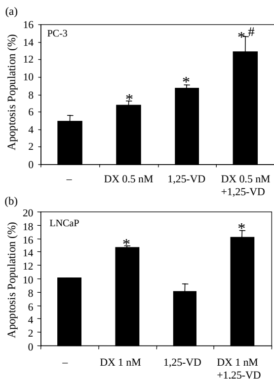
Fig. 3. Pre-treatment with 1,25-VD increases the apoptosis population induced by DX treatment in PC-3 but not LNCaP cells. (a) PC-3 cells were seeded at a density of 2 \times 10^4 in 60-mm dishes and cultured in 10% FBS supplemented RPMI. After 24 h, cells were treated with EtOH or 100 nM 1,25-VD for 2 days. Medium was replaced and cells were treated with or without 0.5 nM DX. After 3 days, the apoptosis populations were assayed and plotted. * P < 0.05 compared with EtOH treated group by using Student's t -test. (b) LNCaP cells were seeded at a density of 10^5 cells in 60-mm dishes and cultured in 10% FBS supplemented RPMI. After 48 h, cells were treated with EtOH or 100 nM 1,25-VD for 1 day. Medium was replaced and cells were treated with or without 1 nM DX. After 3 days, the apoptosis populations were assayed and plotted. * P < 0.05 compared with EtOH treated group, # P < 0.05 compared with DX alone treated group by using Student's t -test.
