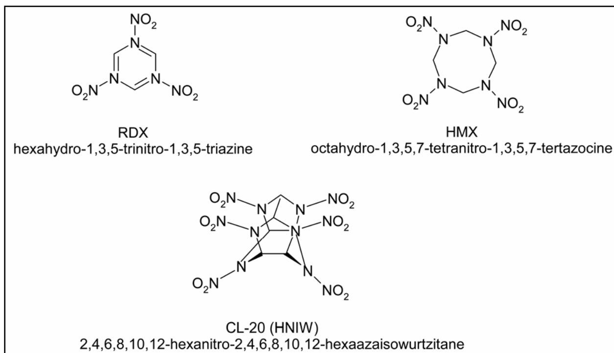
Figure 1. Structure of CL-20 and related nitramines, RDX and HMX.
