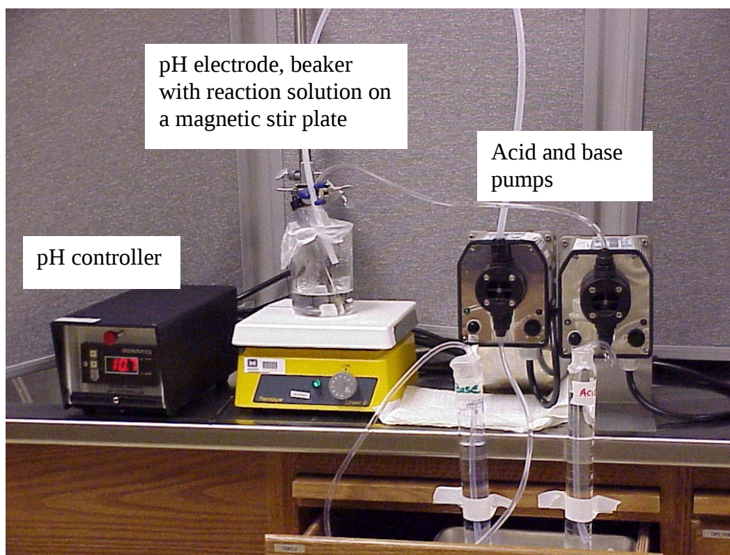
Figure 2. The batch reactor assembly used to track the alkaline hydrolysis of CL-20.
