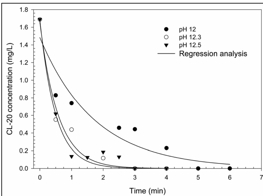
Figure 4. CL-20 concentration profiles at different pH values at an initial concentration of 1.69 mg/L.
