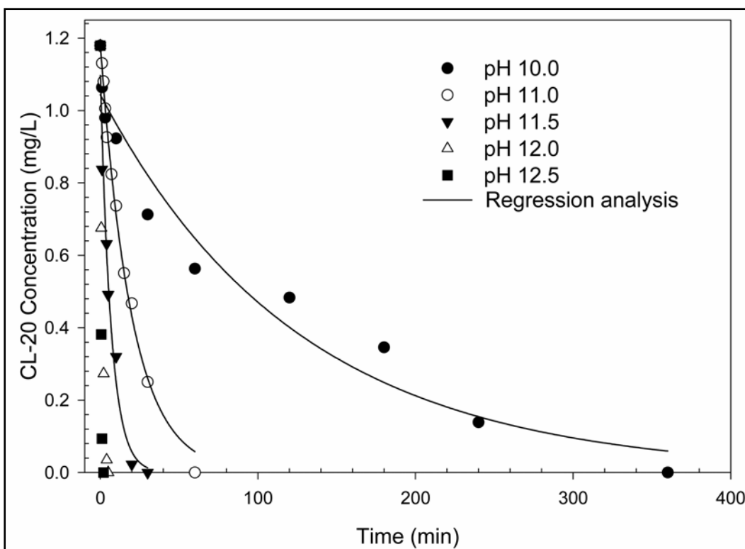
Figure 3. CL-20 concentration profiles at different pH values at an initial concentration of 1.18 mg/L.
