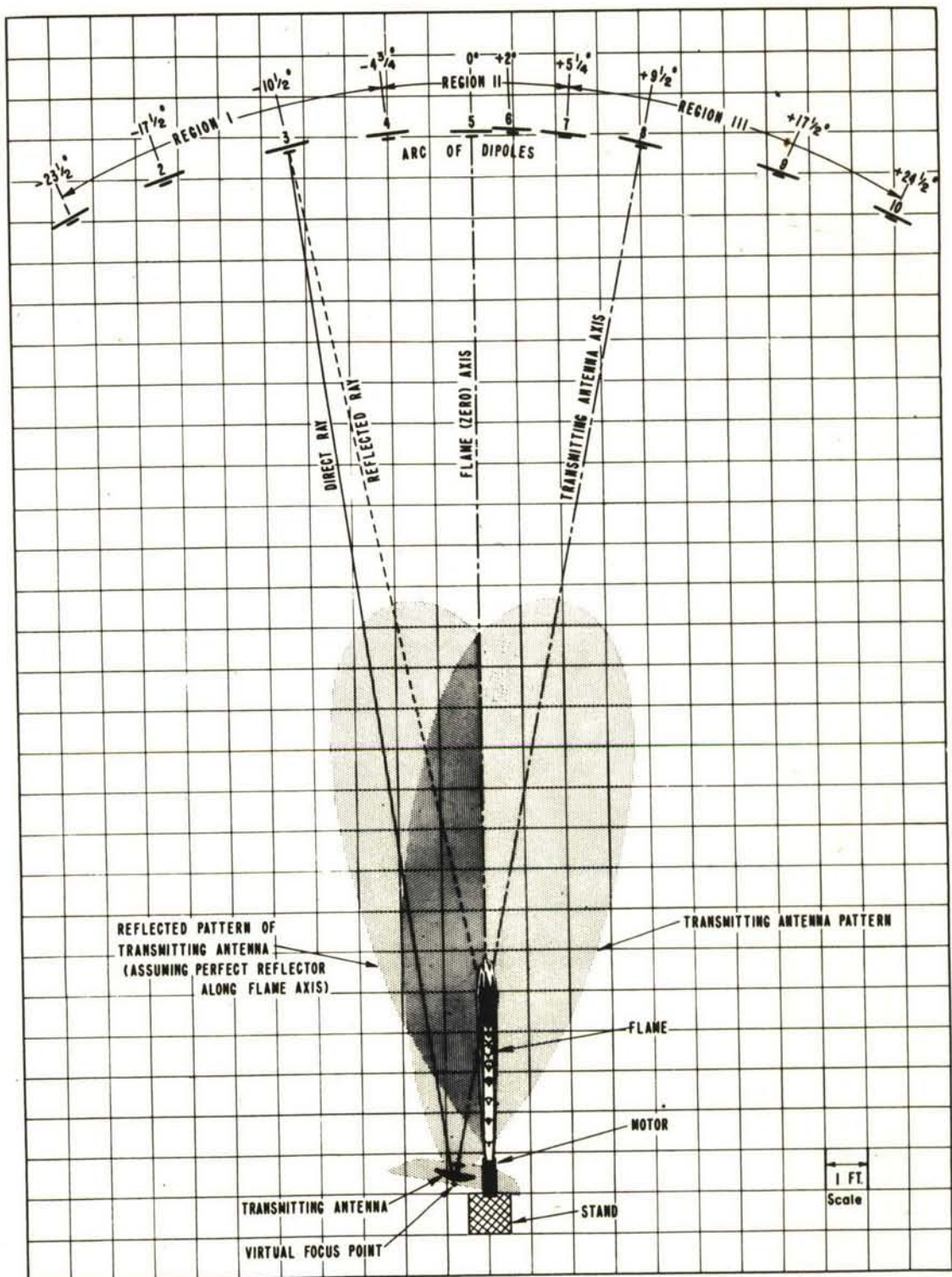
Figure 4 - Diagram (to scale) showing arrangement of propagation
