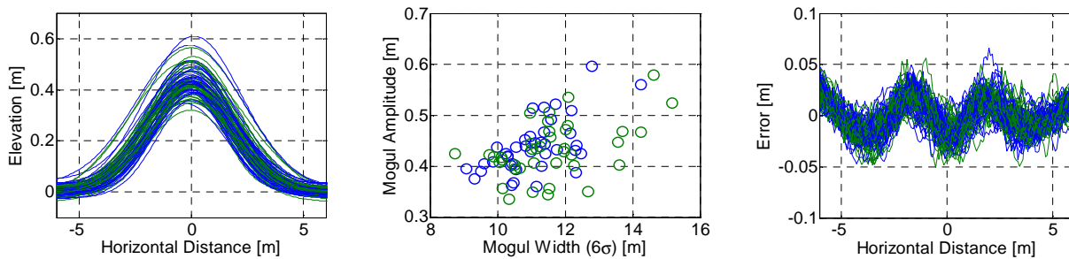
Figure 3. (left) Plot of the Gaussian best fit for the 39 moguls. (middle) Plot of the mogul amplitude ( a ) vs. the mogul width ( 6\sigma ). (right) Plot of the error from the Gaussian best fit. Note scales are not the same.
