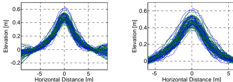
Figure 2. Plot of 39 moguls overlaid. (left) plot over the segment [-9m, 9m]. (right) plot over the horizontal interval [-6m, 6m] for comparison to the fit moguls. Right track traces are in blue and left track traces are in green. Observe that the moguls range in height from 0.36 m to 0.63 m.
