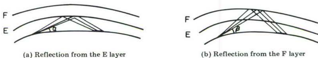
(U) Fig. 5—Reflection of rays
