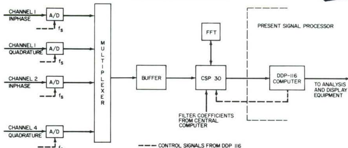
(U) Fig. 7—Preprocessor
