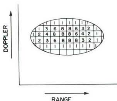
(U) Fig. 3—Target intensity pattern. The numbers within the target outline indicate relative intensity.
