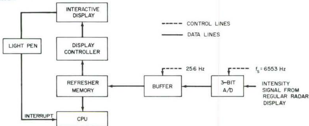
(U) Fig. 2—Dynamic interactive display (with exemplary sampling rates based on a 10-second frame time)
