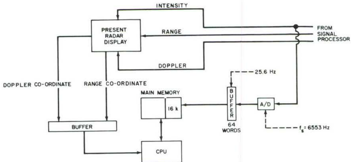
(U) Fig. 4—Target-designation subsystem using a conductive glass overlay
